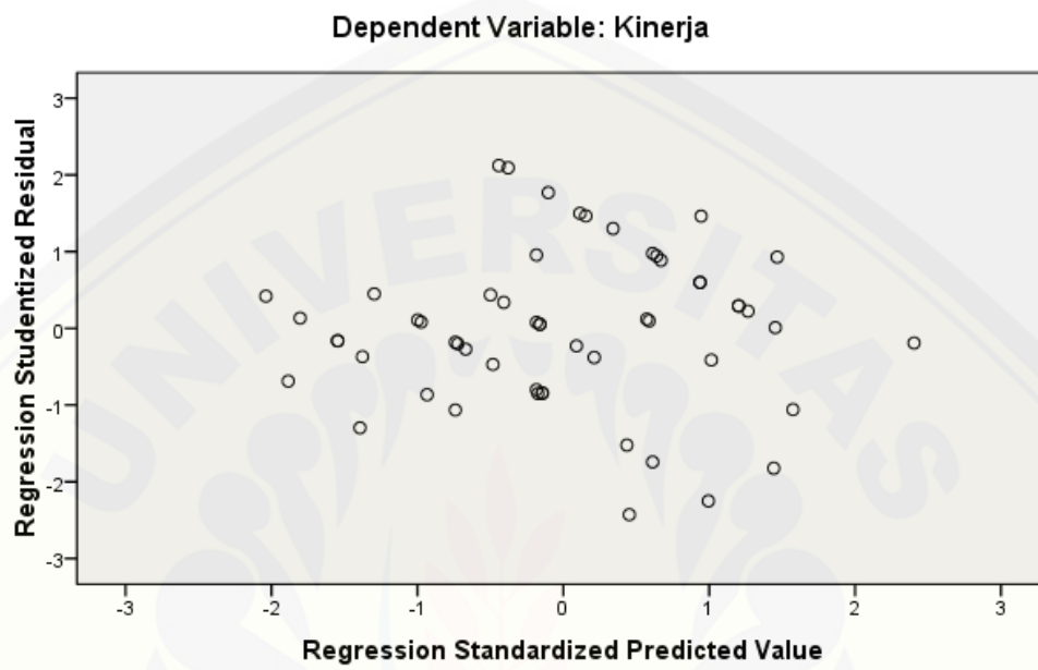
Scatterplot
