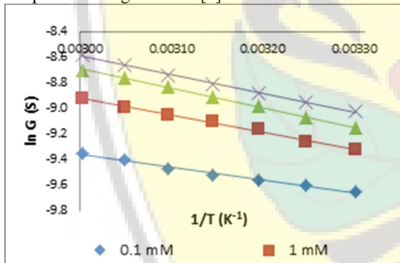
Fig 2. Plot of conductance of various concentration MgCl 2 through the inner membrane of Salak at different temperatures (303-333 K)
