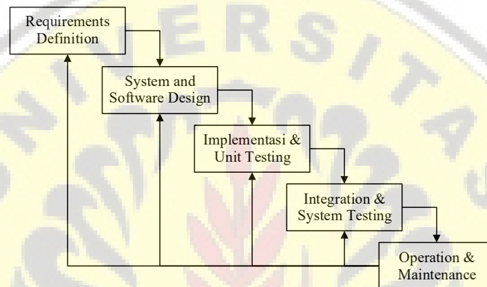
Gambar 1. Model Waterfall
