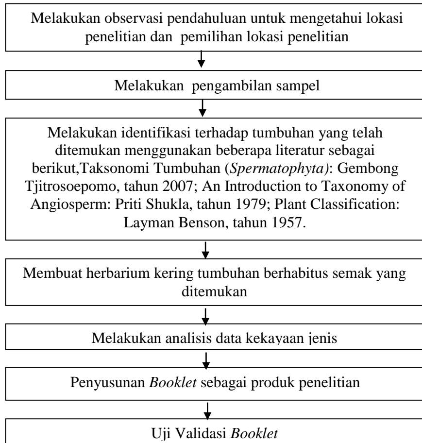
Gambar 3. 4 Alur Penelitian
