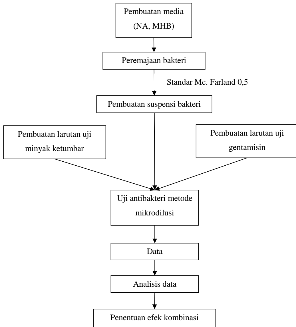
Gambar 3.3 Alur Penelitian
