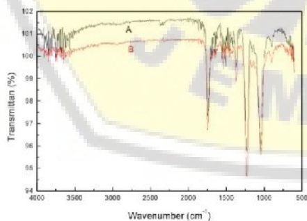
Figure 3. FTIR spectra of (A) the commercial cellulose acetate (CCA); (B) cellulose acetate from bacterial cellulose (CA)
