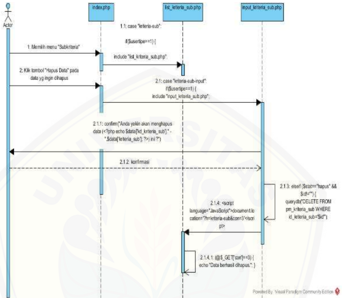
Gambar 36. Sequence Diagram Pengelolaan Data Subkriteria (Hapus Data)
