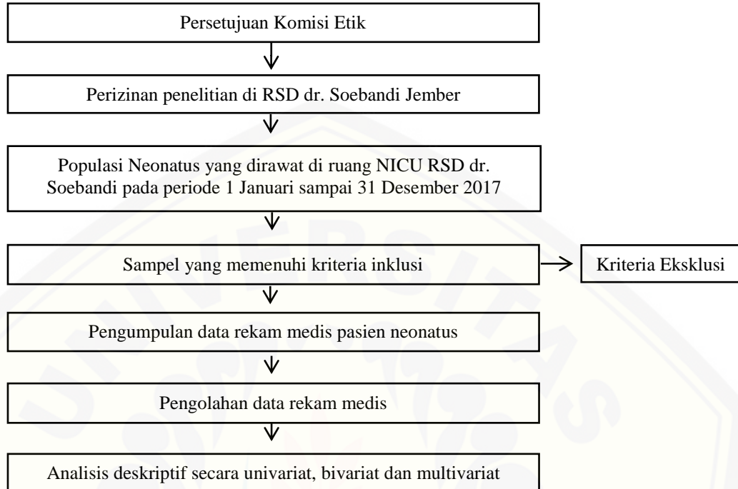
Gambar 3.2 Alur penelitian
