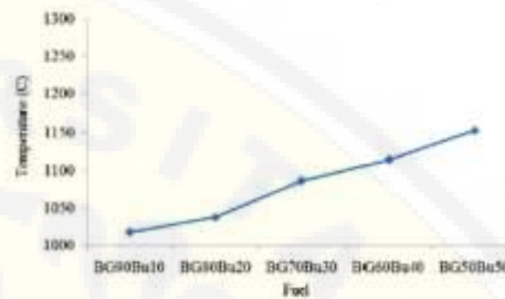
Figure 9 Graph flame temperature of fuel
