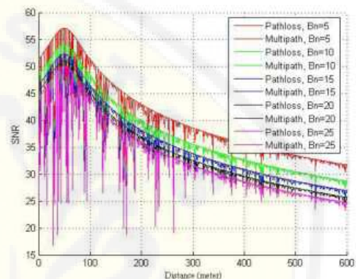
Fig. 5. SNR for Transmitter Power 0.1 Watt
