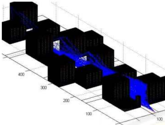
Fig. 1. The Communication System Model at Buildings Environment
