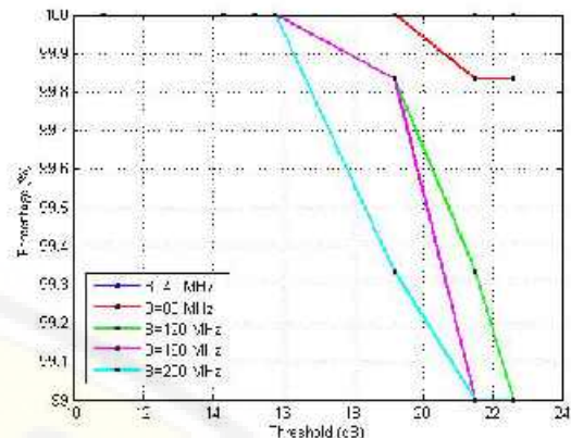
Fig.8. The Coverage Percentage When Transmitter Power 0.1 Watt
