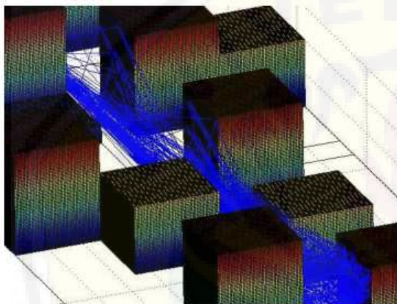
Fig. 2. Multipath Model Around Buildings
