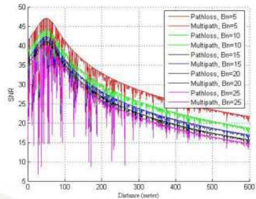
Fig. 4. SNR for Transmitter Power 0.01 Watt
