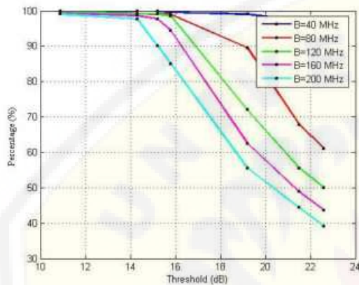
Fig.7. The Coverage Percentage When Transmitter Power 0.01 Watt
