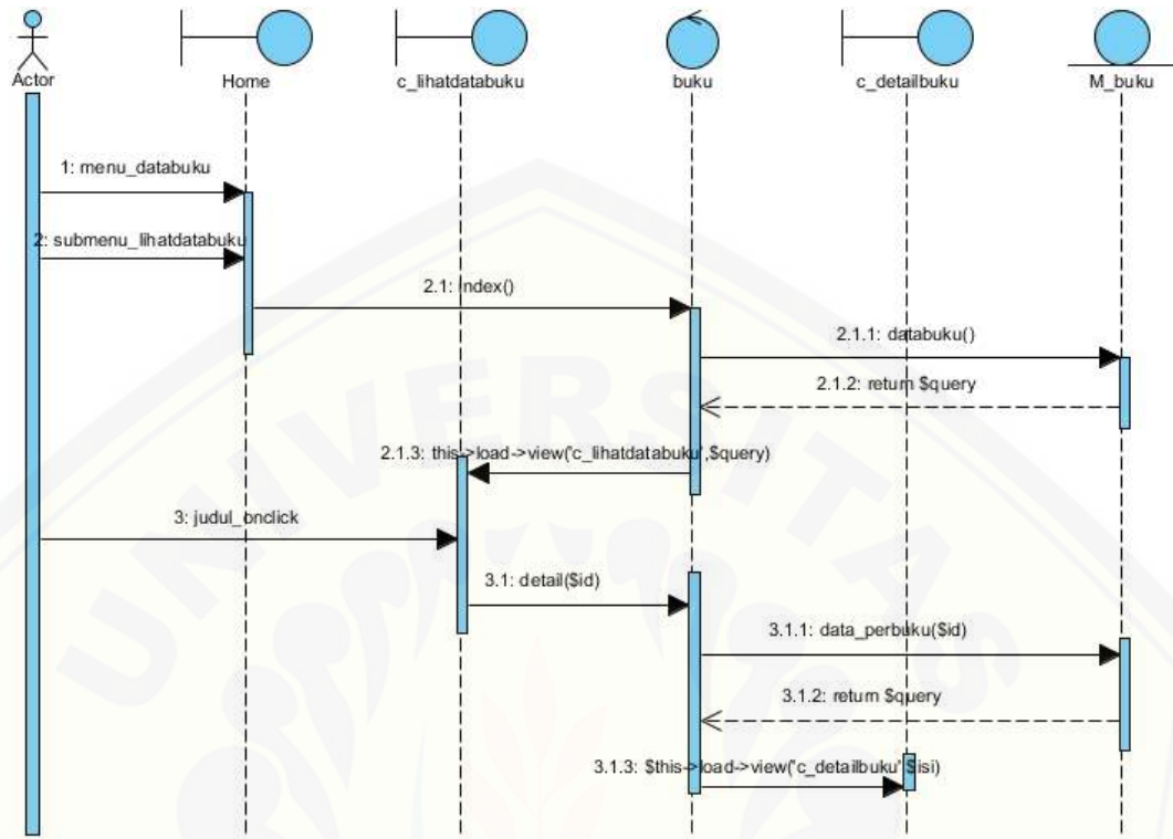
Gambar 4.11 Sequence Diagram Mengelola Data Buku ( view )
