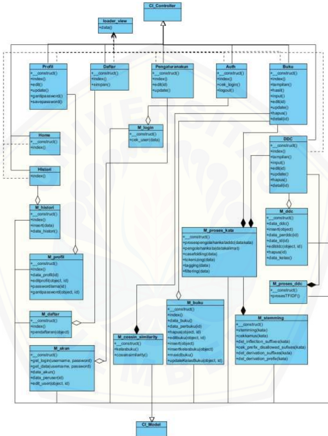
Gambar 4.19 Class Diagram
