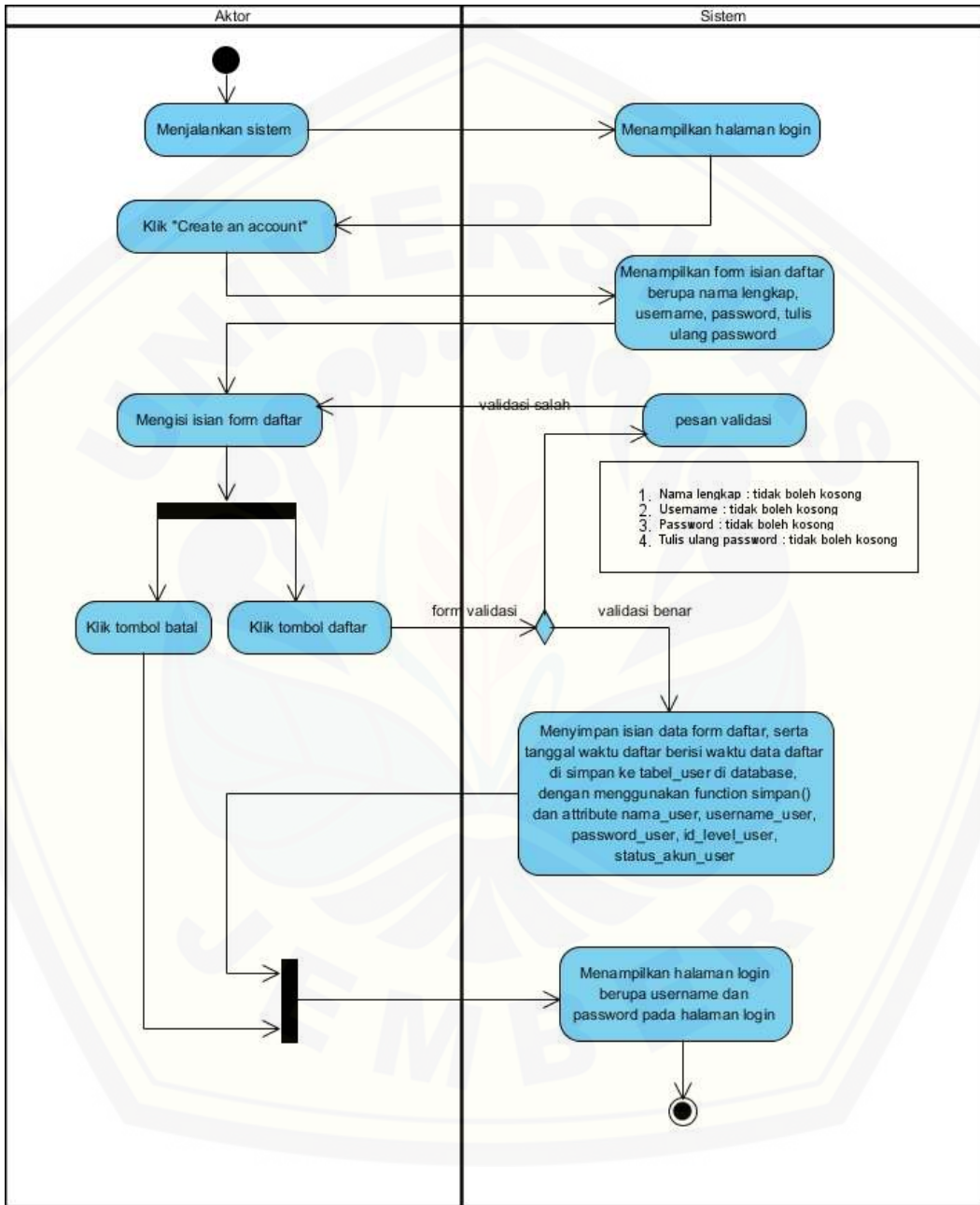
Gambar B.1 Activity Diagram Daftar
