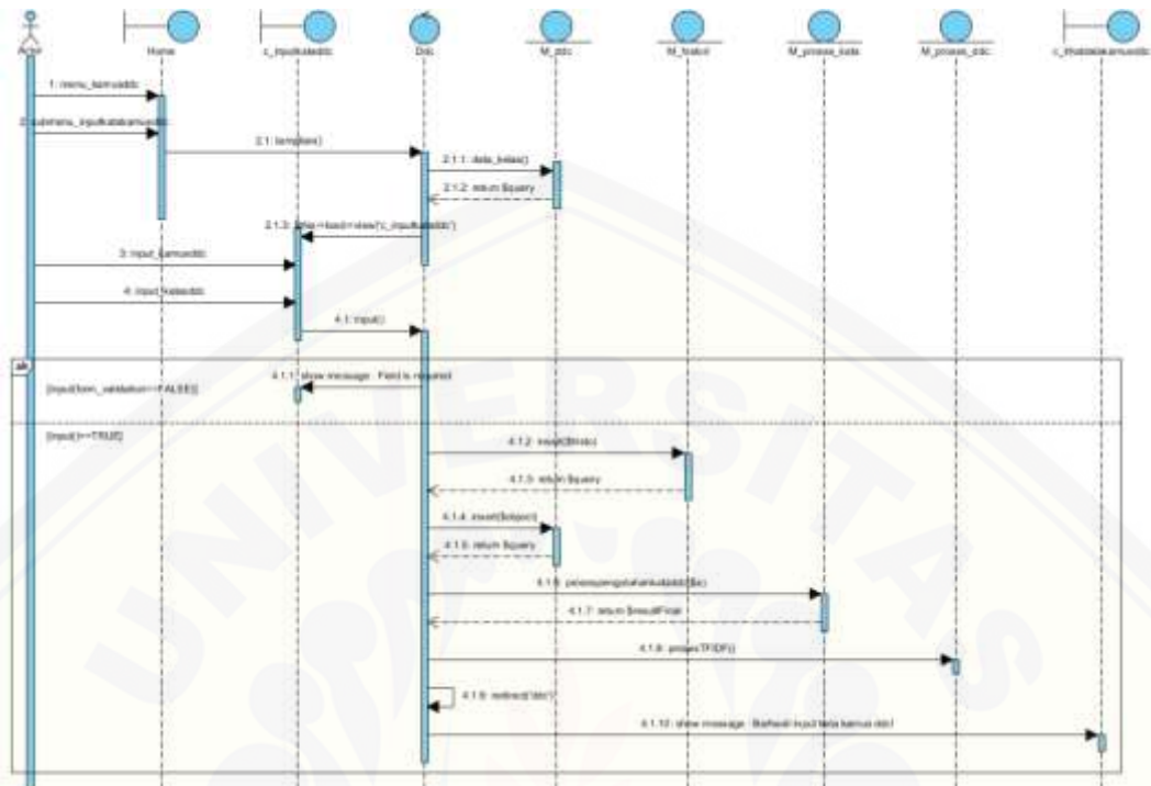
Gambar 4.16 Sequence Diagram Mengelola Data Kamus DDC ( input )
