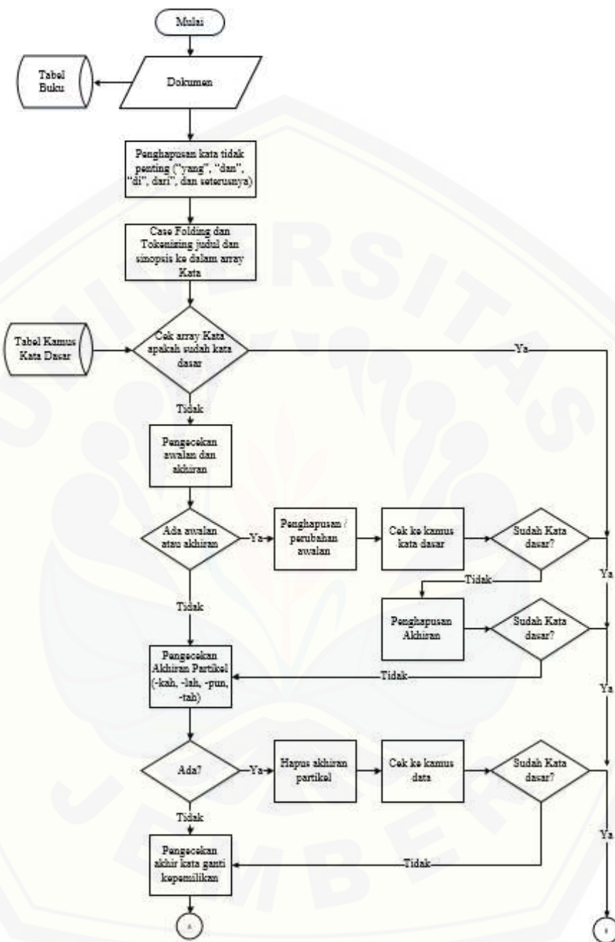
Gambar 3.1 Flow Chart Textmining Bagian 1
