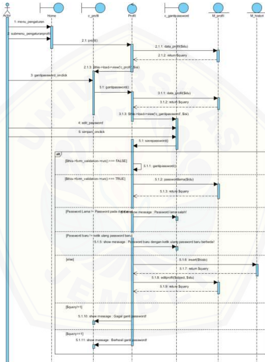
Gambar C.7 Sequence Diagram Mengatur Profil (ganti password)
