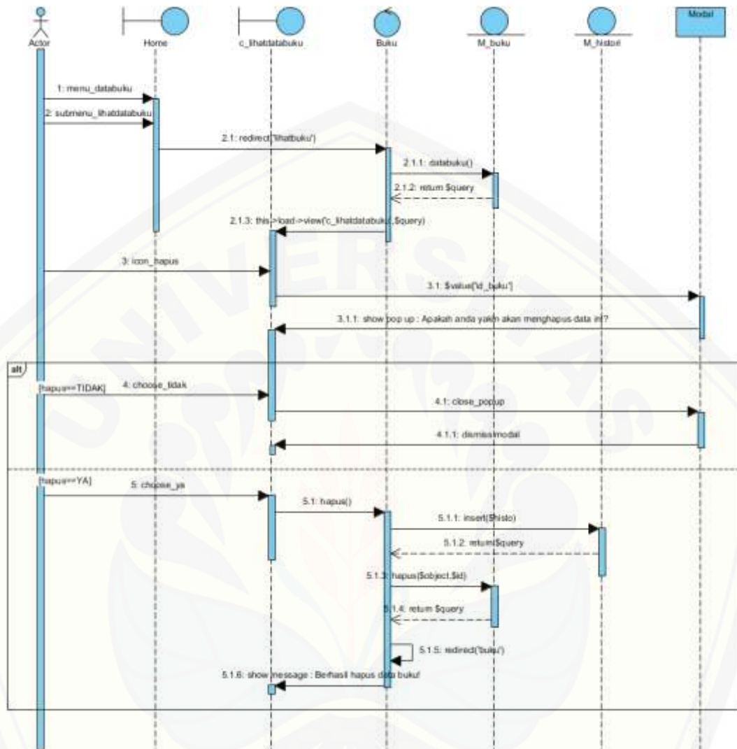
Gambar 4.14 Sequence Diagram Mengelola Data Buku ( delete )
