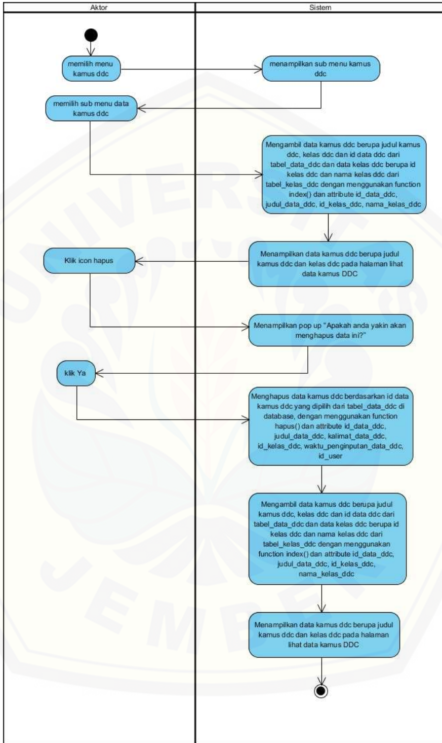
Gambar 4.10 Activity Diagram Mengelola Data Kamus DDC (delete)
