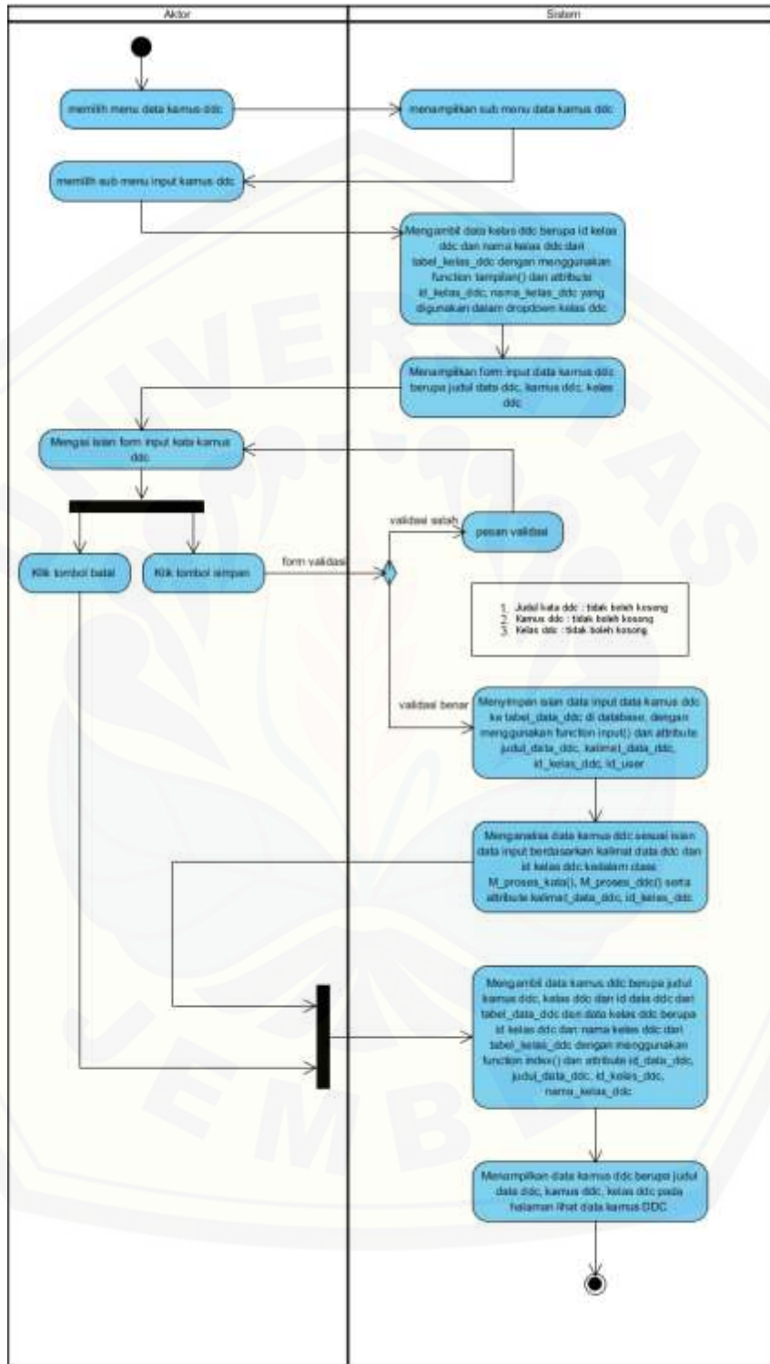
Gambar 4.7 Activity Diagram Mengelola Data Kamus DDC (input)
