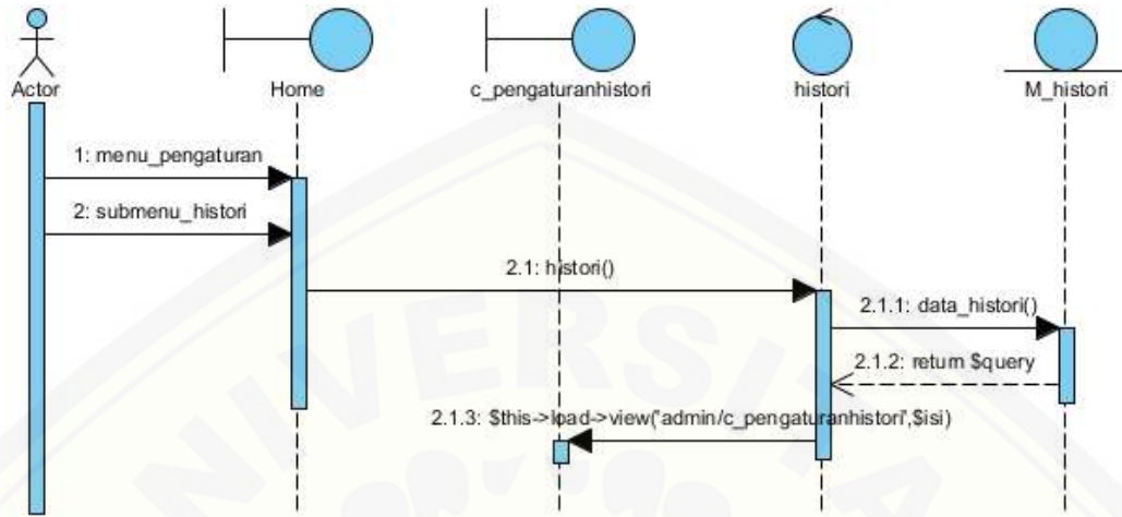
Gambar C.8 Sequence Diagram Melihat Histori
