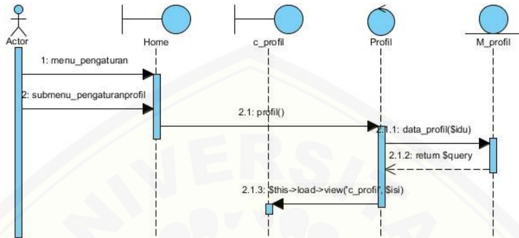
Gambar C.5 Sequence Diagram Mengatur Profil (view)
