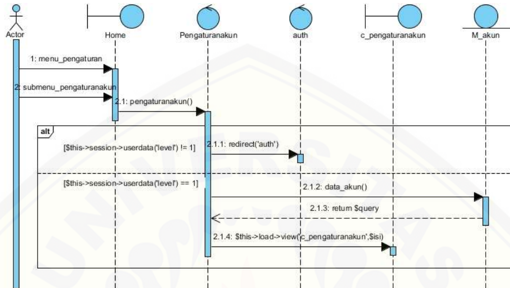
Gambar C.3 Sequence Diagram Mengelola Data Akun (view)
