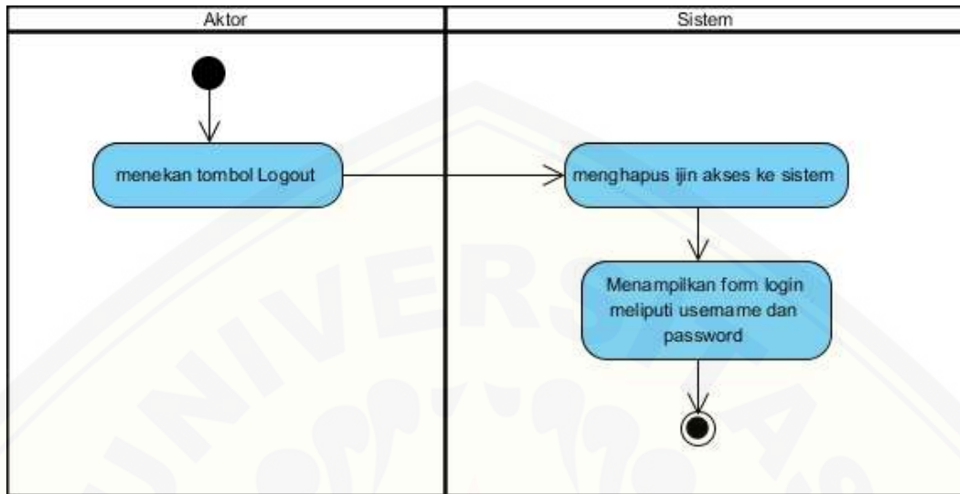
Gambar B.9 Activity Diagram Logout
