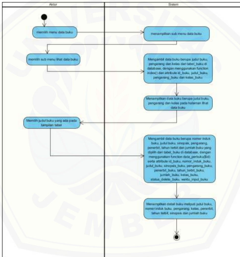
Gambar 4.5 Activity Diagram Mengelola Data Buku ( view )
