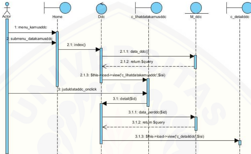
Gambar 4.15 Sequence Diagram Mengelola Data Kamus DDC ( view )
