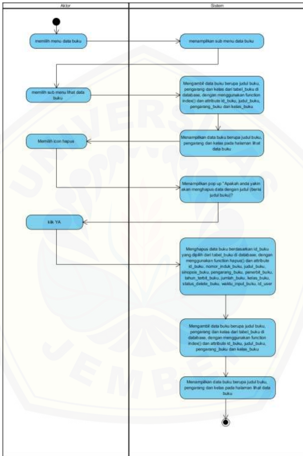
Gambar 4.6 Activity Diagram Mengelola Data Buku (delete)
