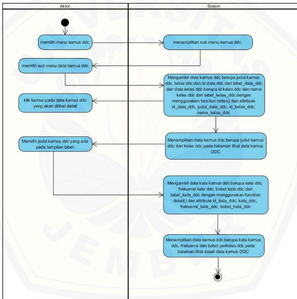
Gambar 4.9 Activity Diagram Mengelola Data Kamus DDC ( view )
