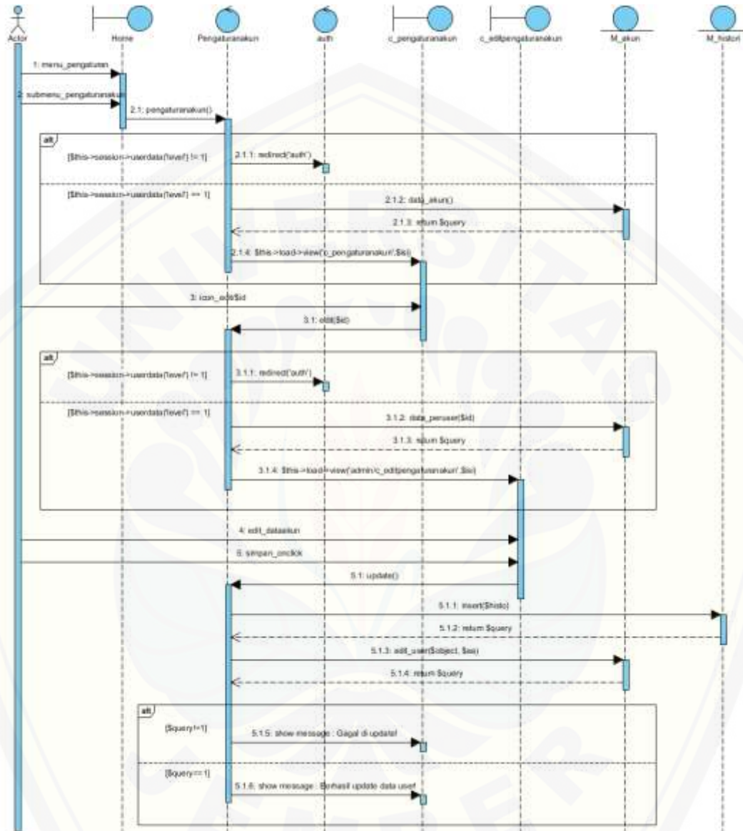
Gambar C.4 Sequence Diagram Mengelola Data Akun ( edit )
