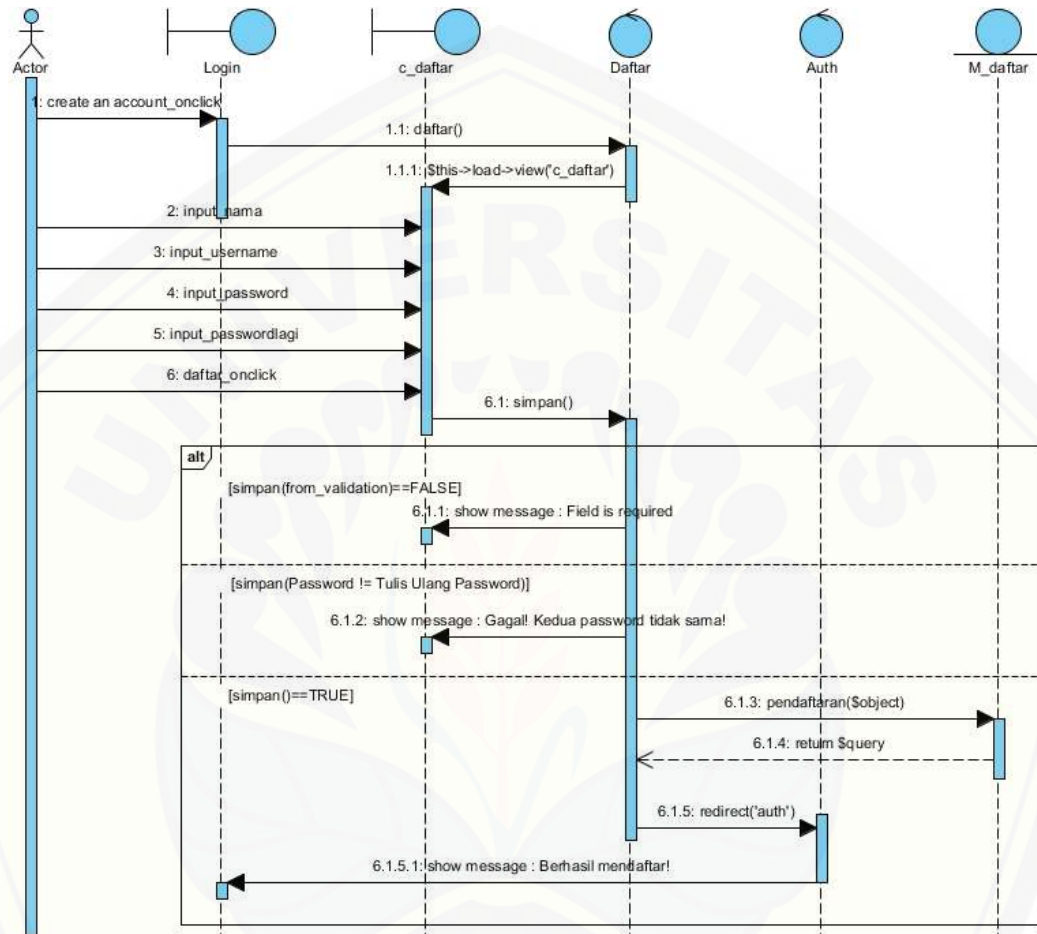
Gambar C.1 Sequence Diagram Daftar
