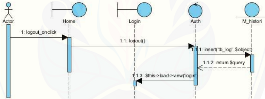
Gambar C.9 Sequence Diagram Logout
