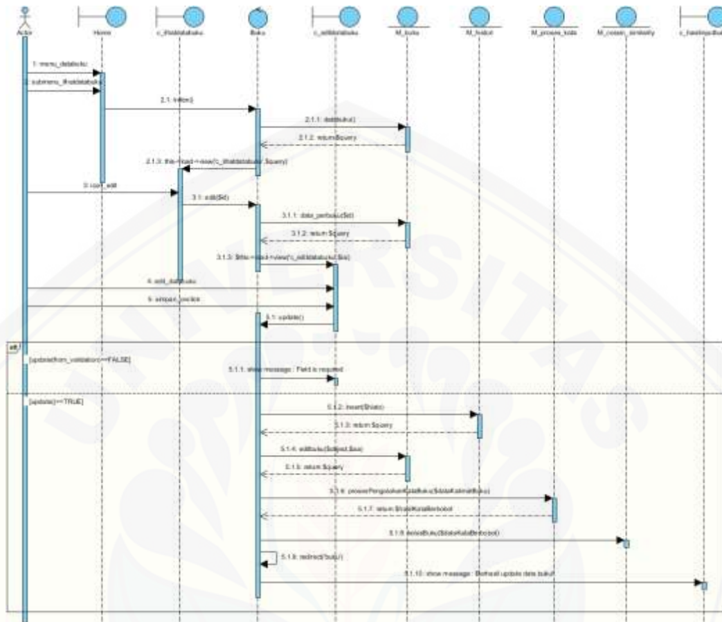
Gambar 4.13 Sequence Diagram Mengelola Data Buku ( edit )
