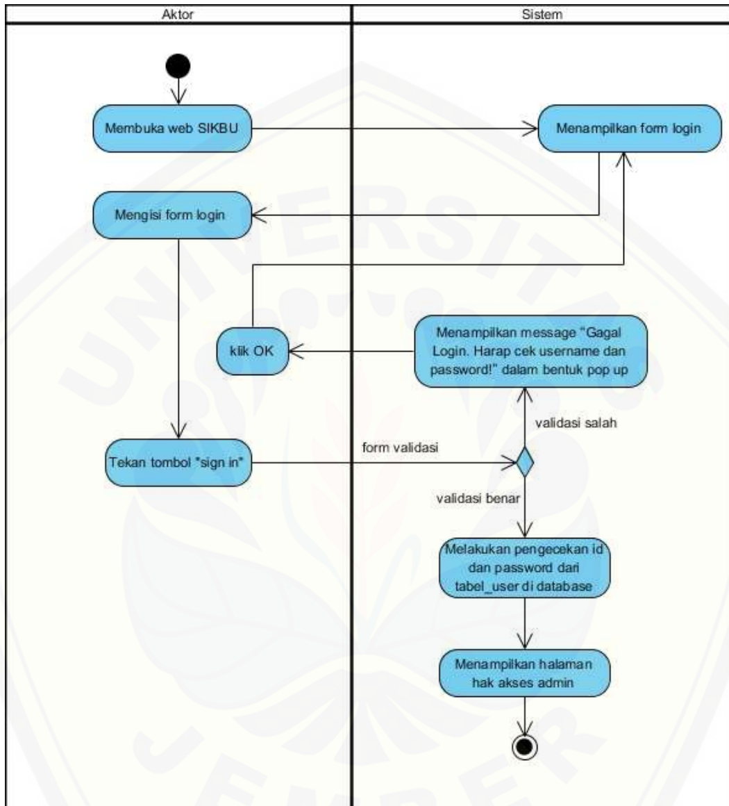
Gambar B.2 Activity Diagram Login
