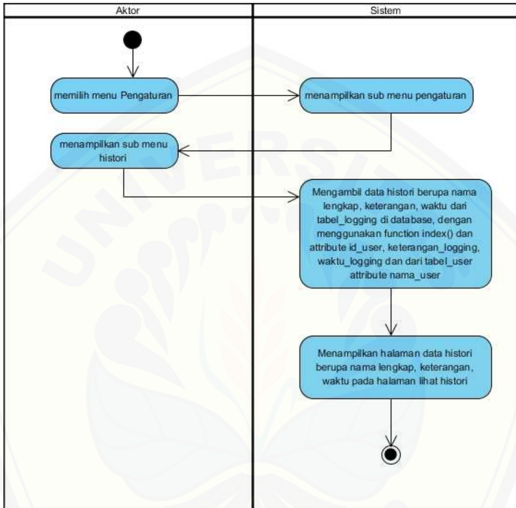
Gambar B.8 Activity Diagram Melihat Histori
