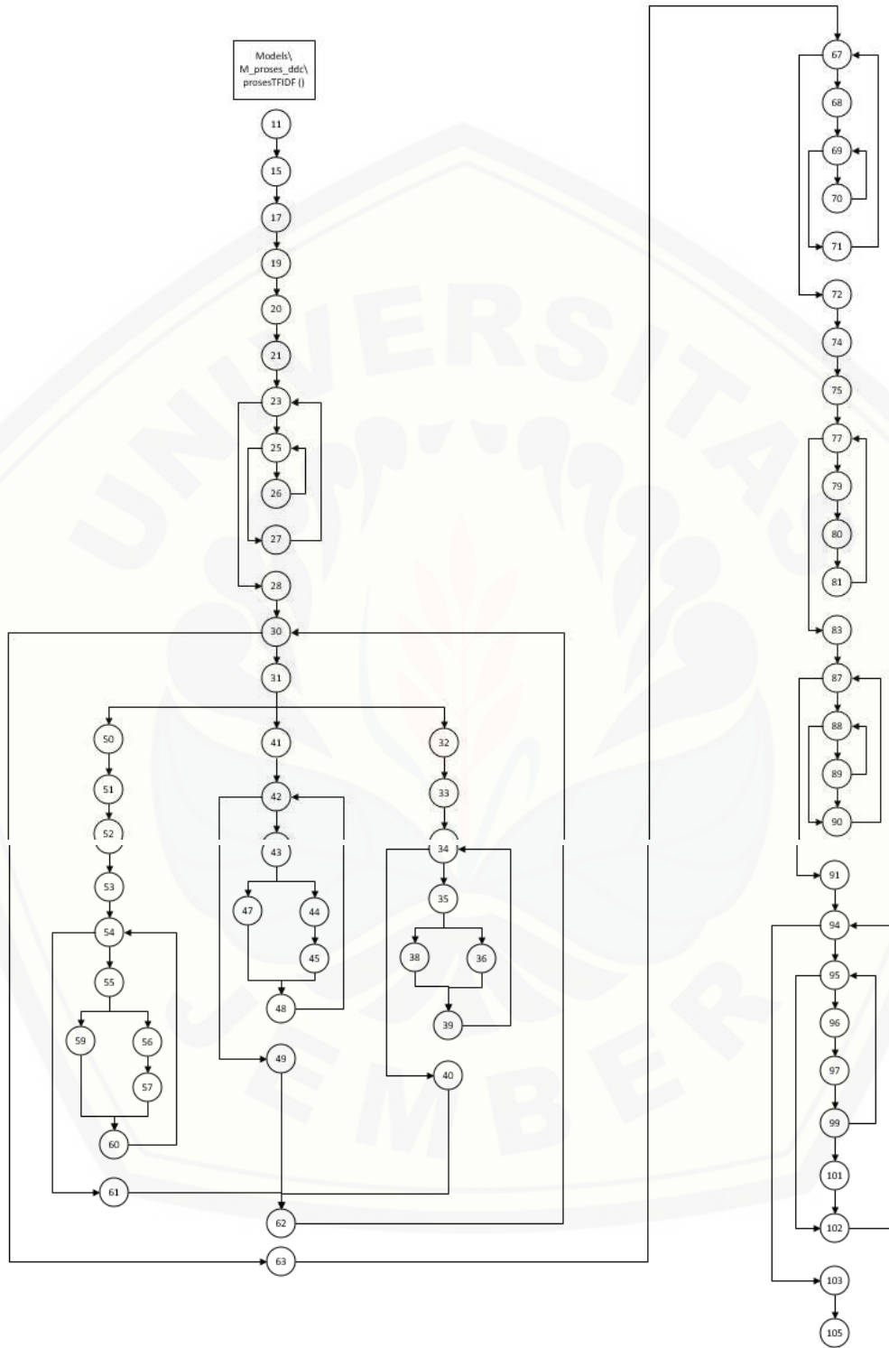
Gambar 4.40 Diagram Alir Function prosesTFIDF()
