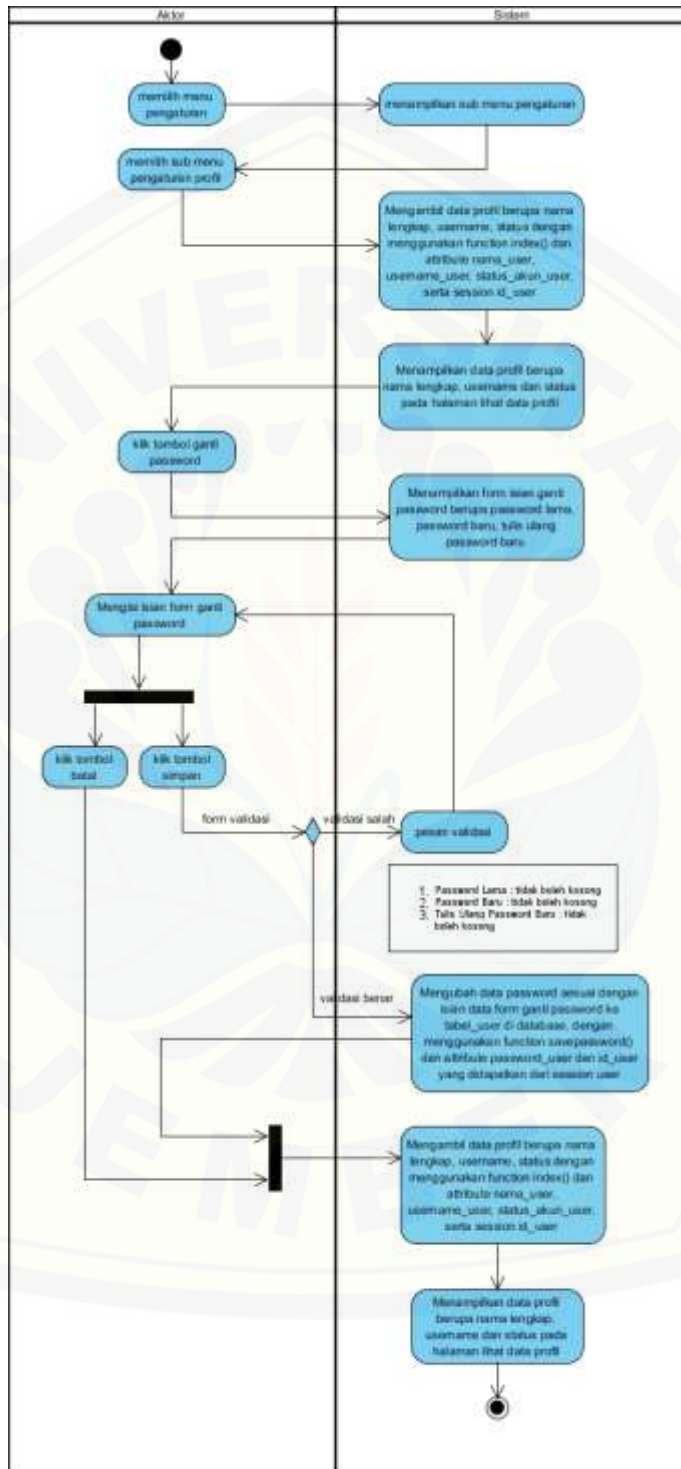
Gambar B.7 Activity Diagram Mengatur Profil (ganti password)
