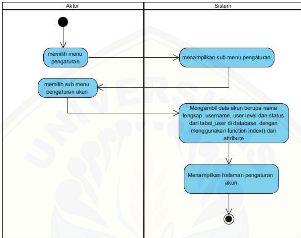
Gambar B.3 Activity Diagram Mengelola Data Akun ( view )
