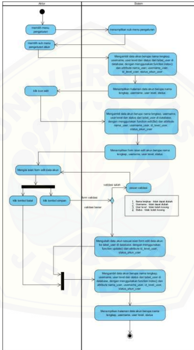
Gambar B.4 Activity Diagram Mengelola Data Akun ( edit )
