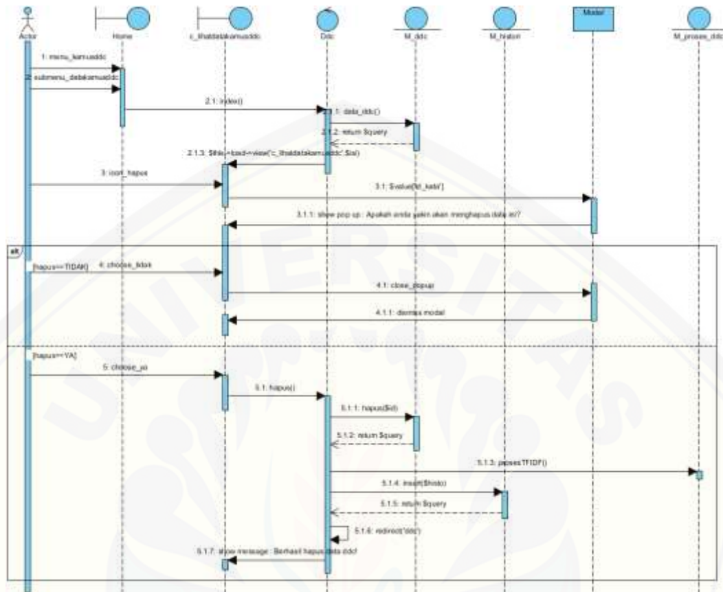
Gambar 4.18 Sequence Diagram Mengelola Data Kamus DDC ( delete )
