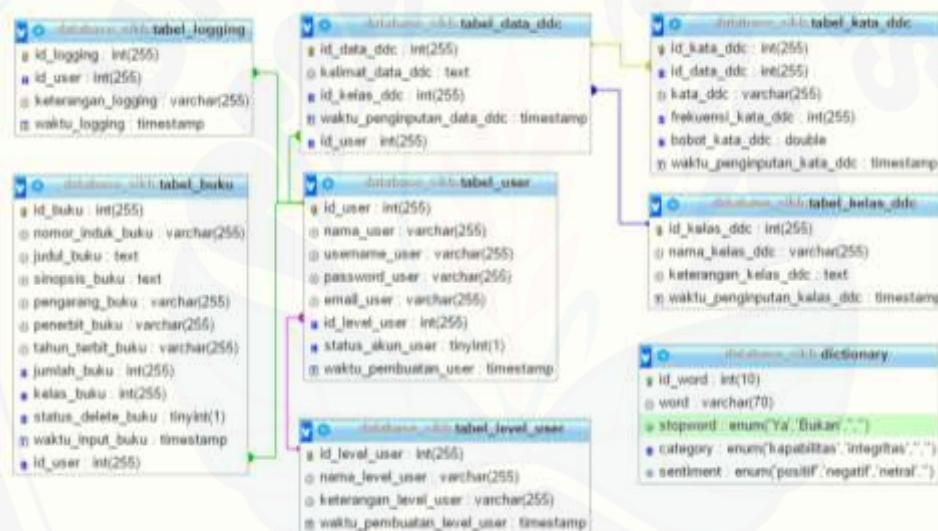
Gambar 4.20 Entity Relational Diagram
