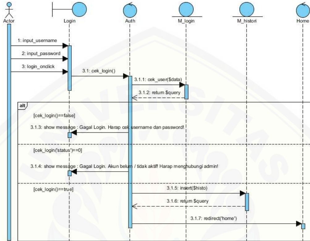
Gambar C.2 Sequence Diagram Login
