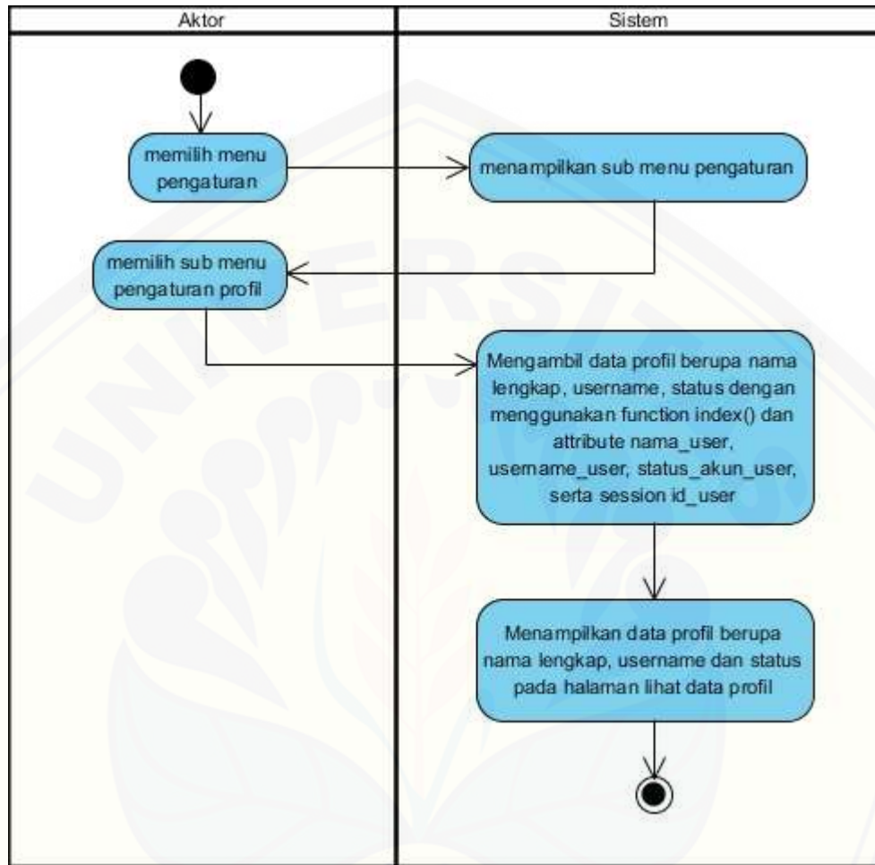
Gambar B.5 Activity Diagram Mengatur Profil ( view )
