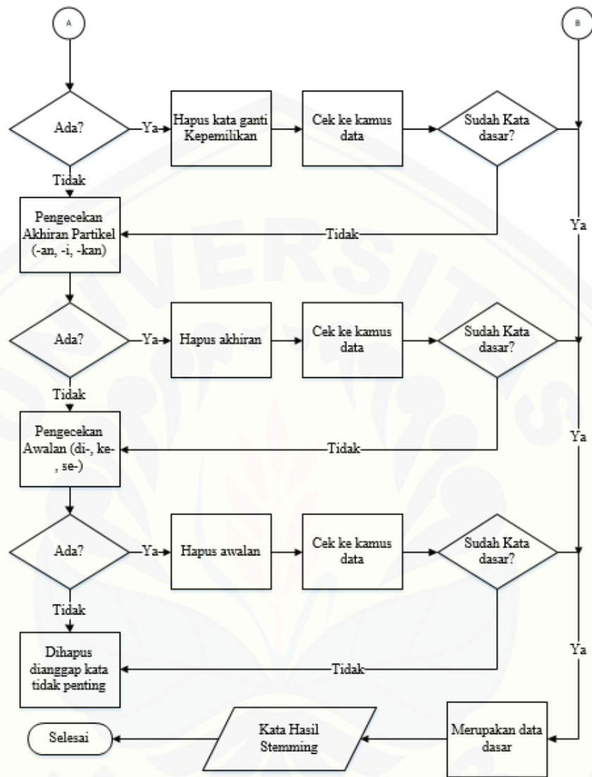
Gambar 3.2 Flow Chart Textmining Bagian 2
