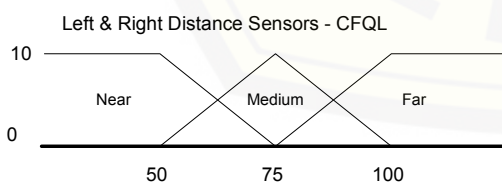
Figure 7. Membership function of left & right distance sensor - CFQL
