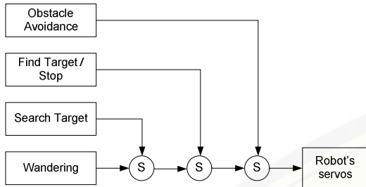
Figure 1. Subsumption Architecture for autonomous navigation robot
