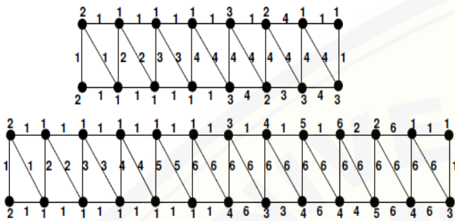
Figure 1: The vertex irregular total labeling of triangular ladder TL_8 and TL_{13}
