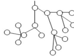
Gambar 3.1 Sampel Snowball
