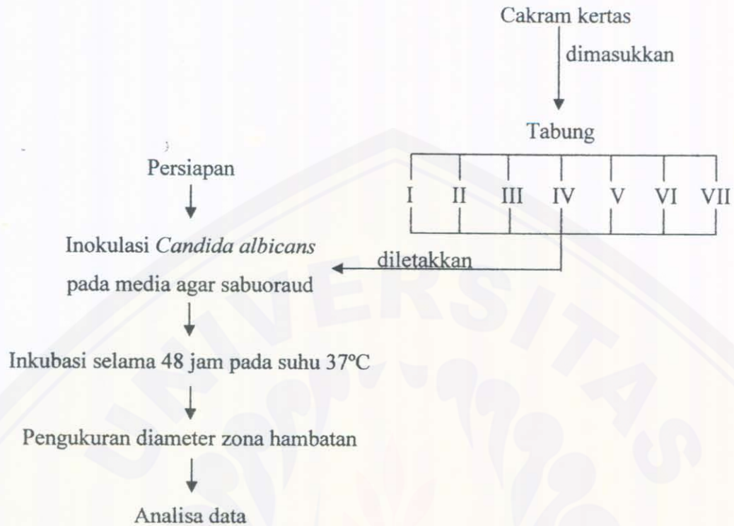
Gambar 3. Alur Penelitian
