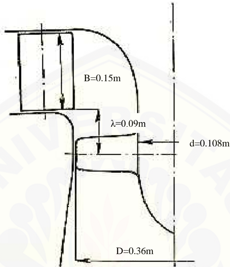
Gambar 4.3 Desain Dimensi Ruang Runner
