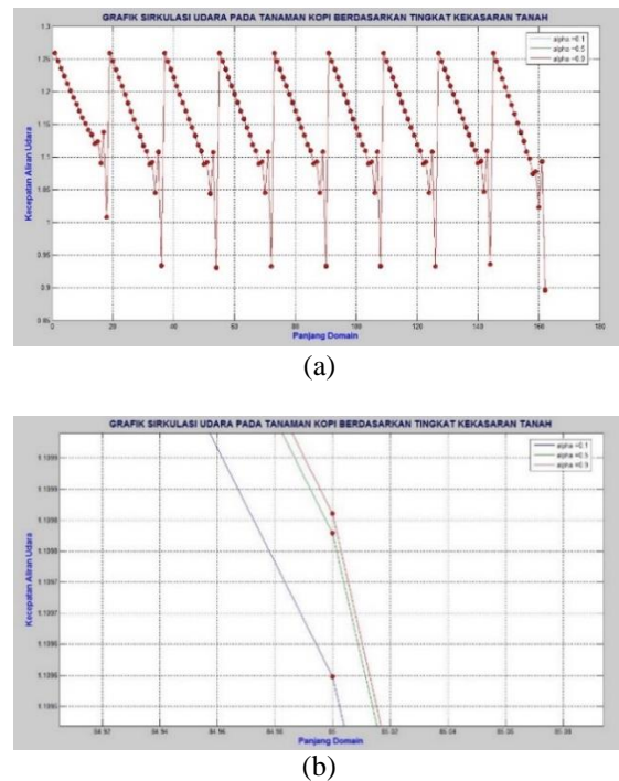
Figure 2. The air circulation on coffee plantation with different level of soil roughness by MATLAB
