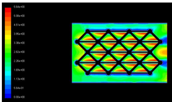
Figure 4. The air circulation on coffee plantation based on cropping patterns of shackle of wheel graph
