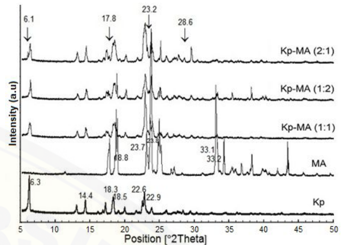
Fig 5. PXRD pattern of Kp, MA and Kp-MA cocrystal at different stoichiometric ratio
