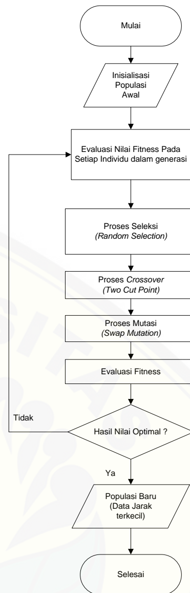
Gbr. 1 Flowchart Metode Algoritma Genetika
