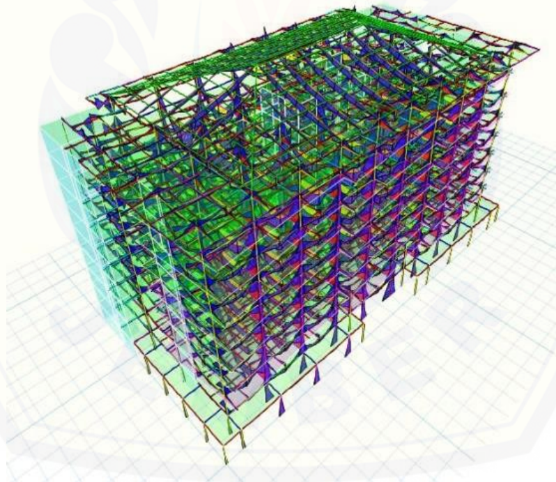
Gambar 4. Diagram gaya momen
