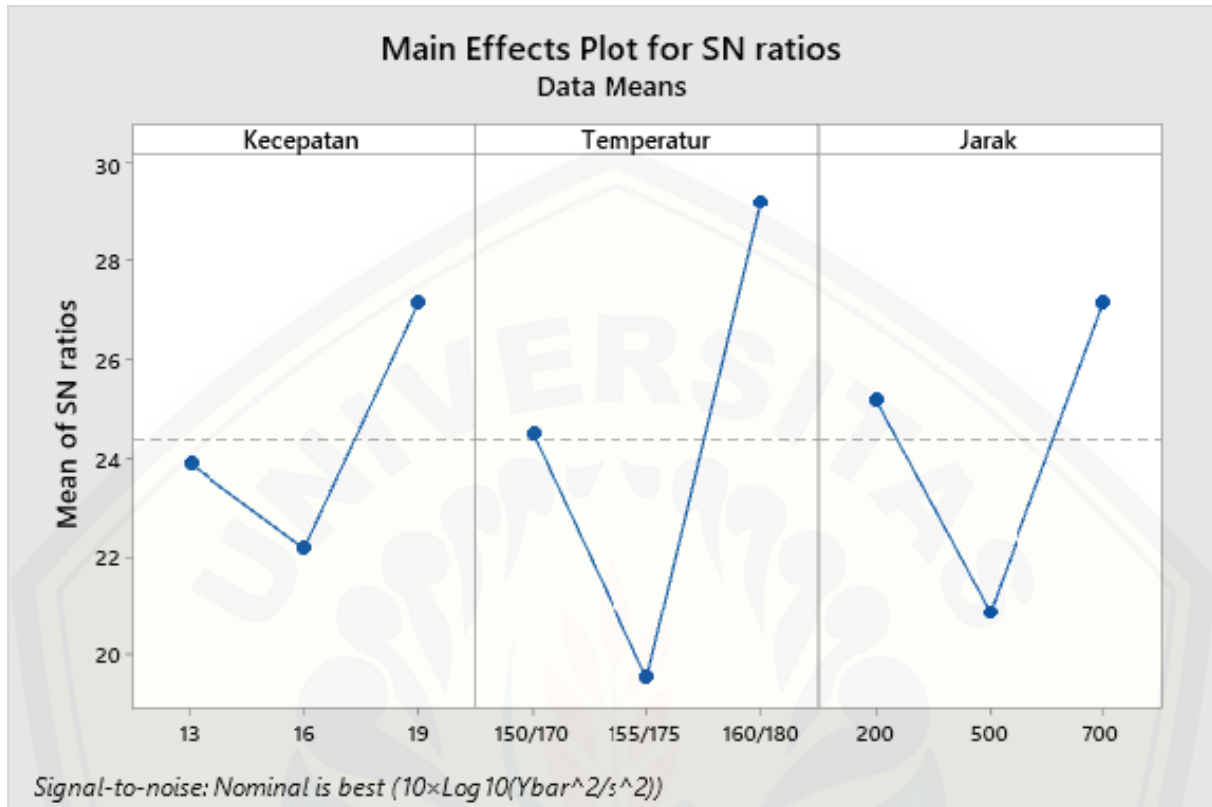
Gambar 3. Plot for S/N Ratio (Minitab 19) Sumber: analysis data (2021).
