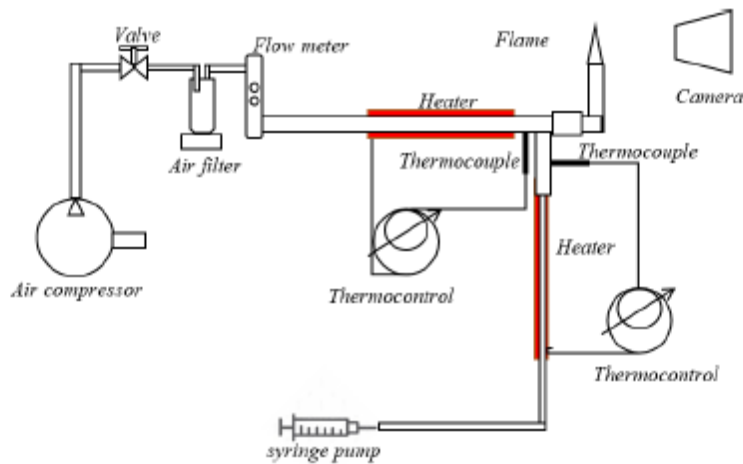
Figure 2. Schematic diagram of the test setup
