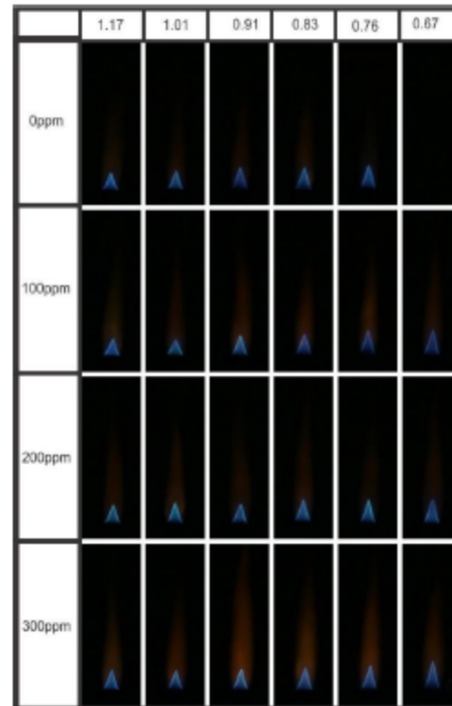
Figure 5. Photo of the experimental bunsen flame
