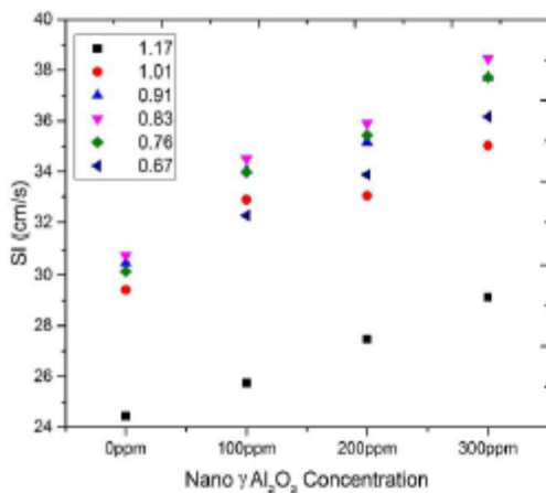
Figure 9. SI vs γ-Al 2 O 3 nano particles concentration
