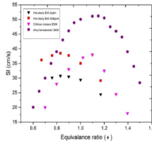
Figure 8. Comparison of laminar flame speeds
