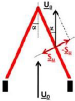
Figure 3. Illustration of cone bunsen flame angle [36]
