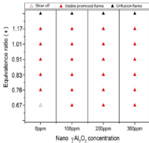
Figure 6. Flame stability map
