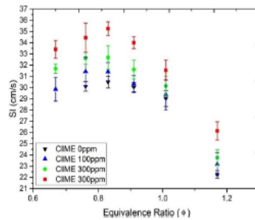
Figure 7. Laminar flame speed of biodiesel and mixture
