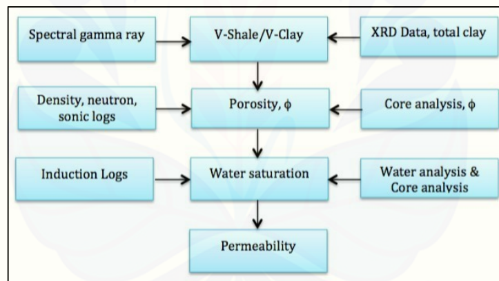
FIGURE 2. Workflow for petrophysical evaluation of tight sand reservoir
