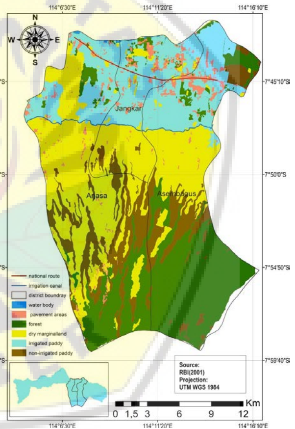
Fig. 6. RBI map; source: own study
