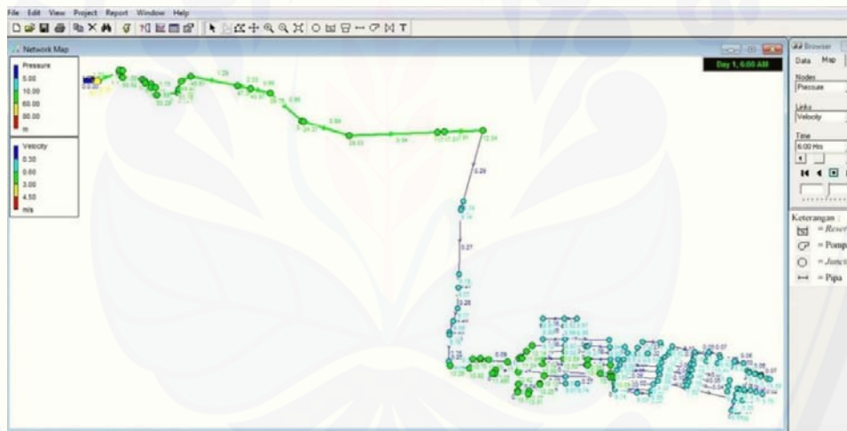
Figure 5. Results of Running the Final Stage Development Modelling for the Drinking Water Distribution Network for Kaliwates Sub-District.
