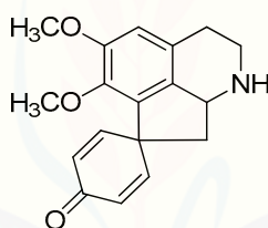
stepharinine 14
