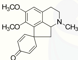
pronuciferine 13
