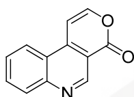
cherimoline 25
