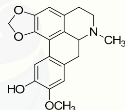
phanostenine 15
