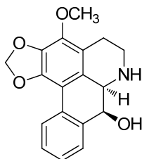
artabonatine B 23
