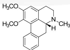
(-)-nuciferine 35
