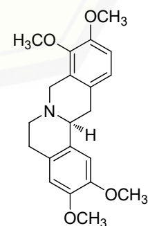
(-)-tetrahydropalmatine 36
