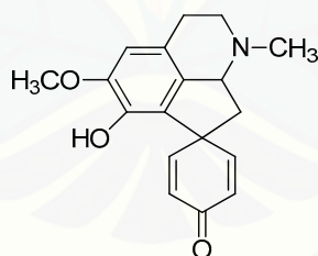
(+)-glaziovine 32
