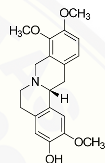
(-)-corypalmine 30
