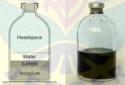
Figure 1. Example of an Assay Vessel for Anaerobic Biodegradability Test (Angelidaki et al., 2007).
