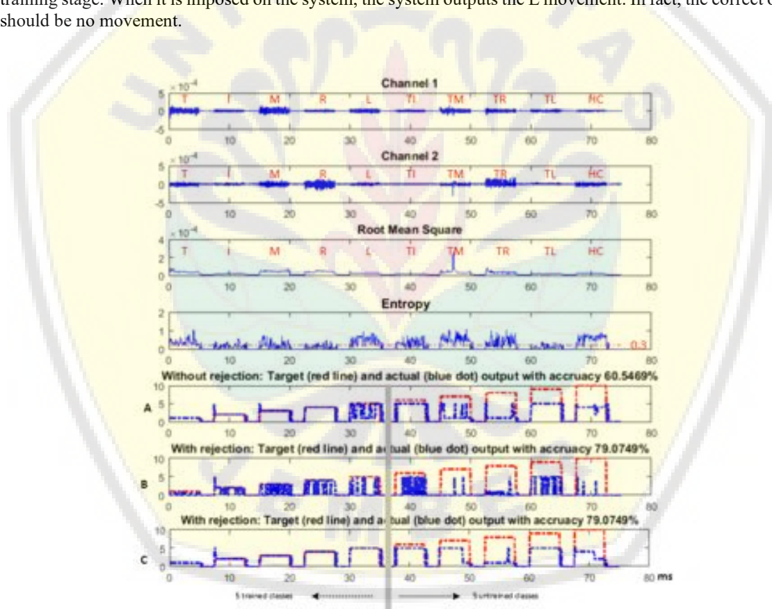
Figure 9. Real-time experiment results over time using threshold 0.3 using 5 trained classes and 5 untrained classes
