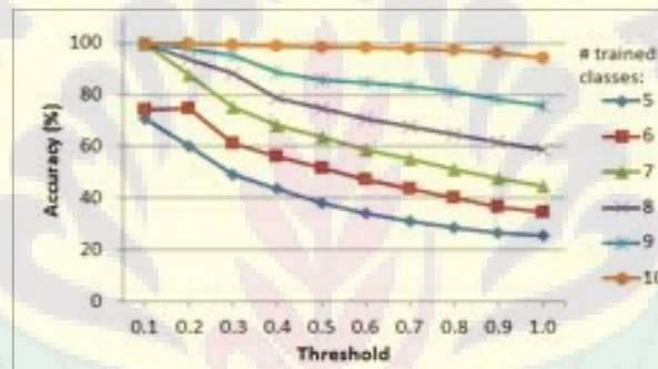
Figure 5. Variation of rejection threshold on the system performance without majority vote
