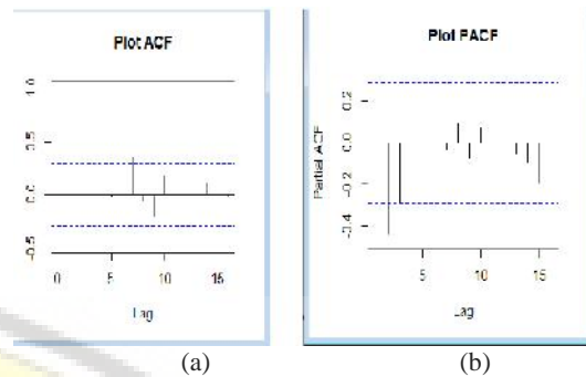
Gambar 1. Plot ACF dan PACF data hasil differencing
