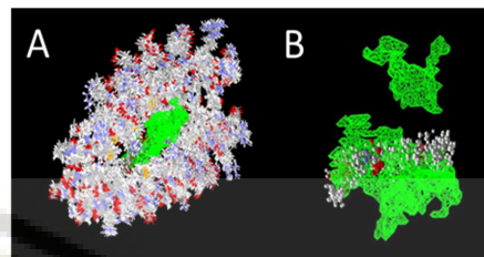
Fig. 1. A. Cavity 1 position in TRPV1 protein (2N27) was shown as the green area, B. The binding site of capsaicin in the cavity 1
