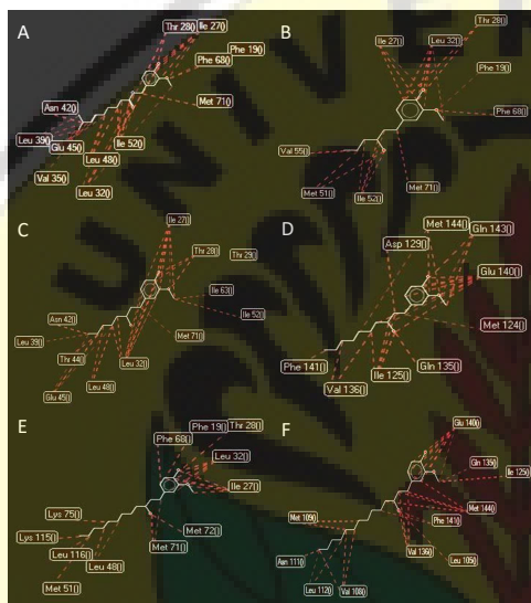
Fig. 4. Steric interactions of A. Capsaicin, B. 2-paradol, C. 4-paradol, D. 6-paradol, E. 8-paradol and F. 10-paradol
