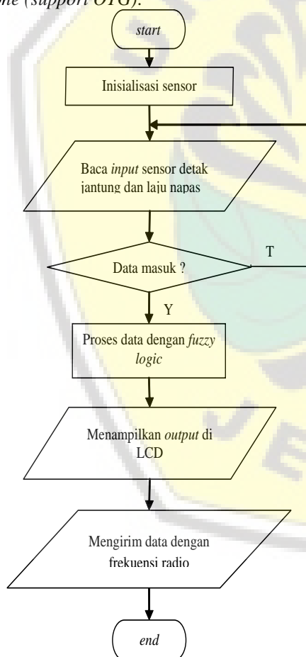
Gambar 16. Flowchart
