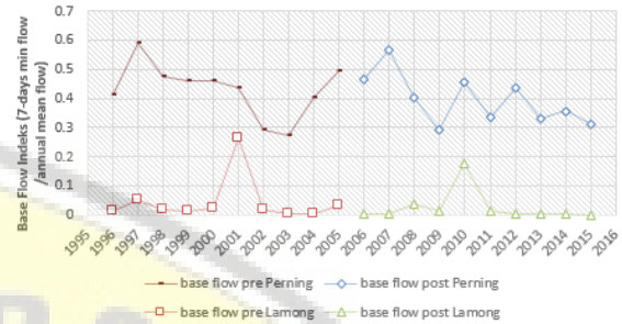
Gambar 13. Base flow indeks
