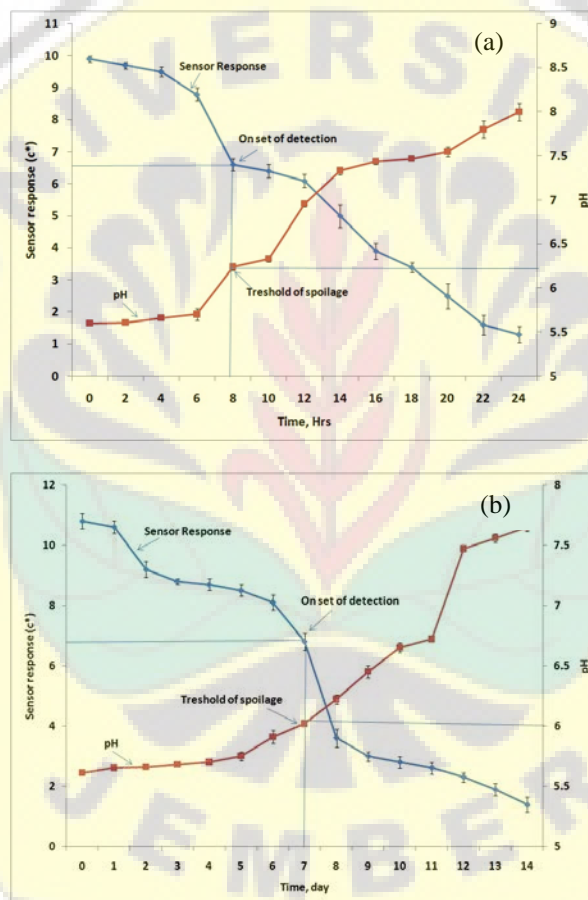
Figure 3 pH values of beef samples and sensor response at room (a) and chiller (b) temperature.
