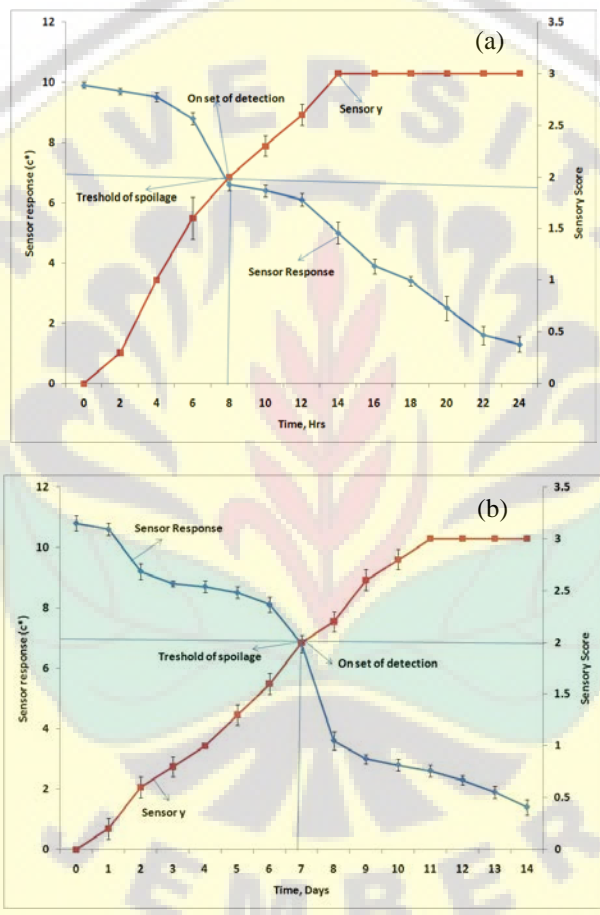
Figure 6 Sensory score of beef samples and sensor response at room (a) and chiller (b) temperature.
