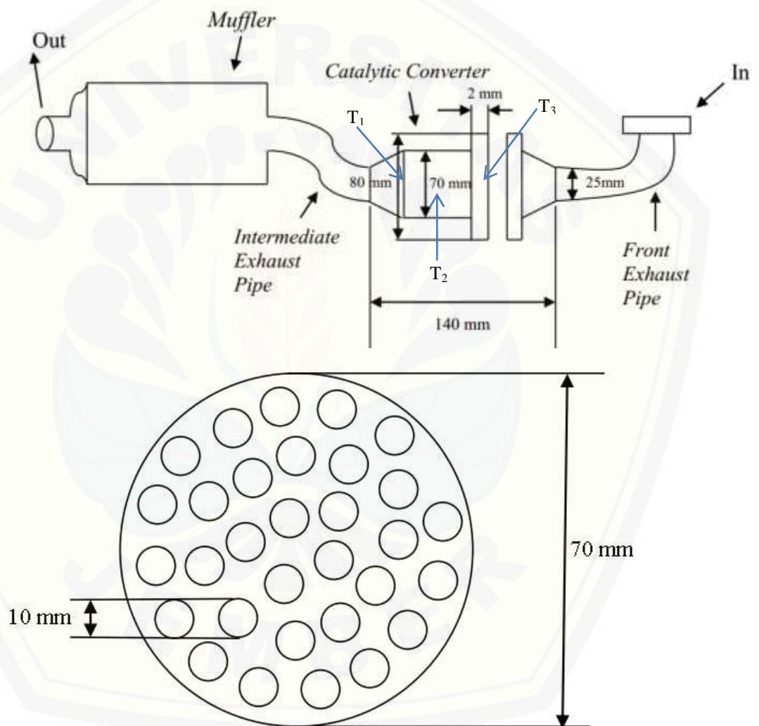
Gambar 3.1 Desain catalytic converter
