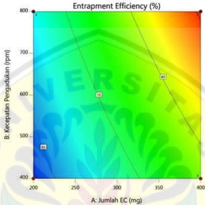
Gambar 2. Hasil Contour plot EE
