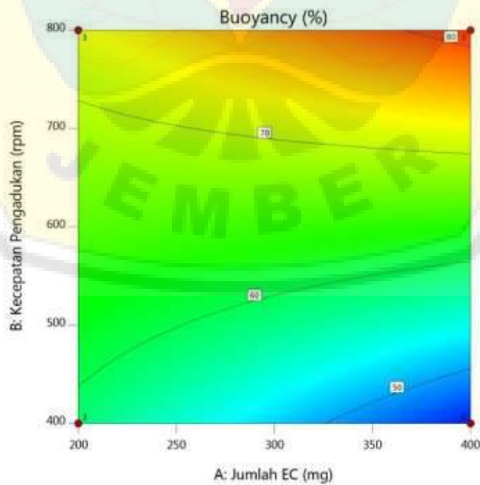
Gambar 3. Hasil Contour plot buoyancy
