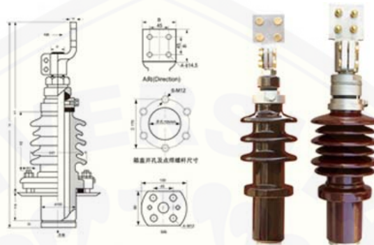
Gambar 2.3. Bushing transformator
