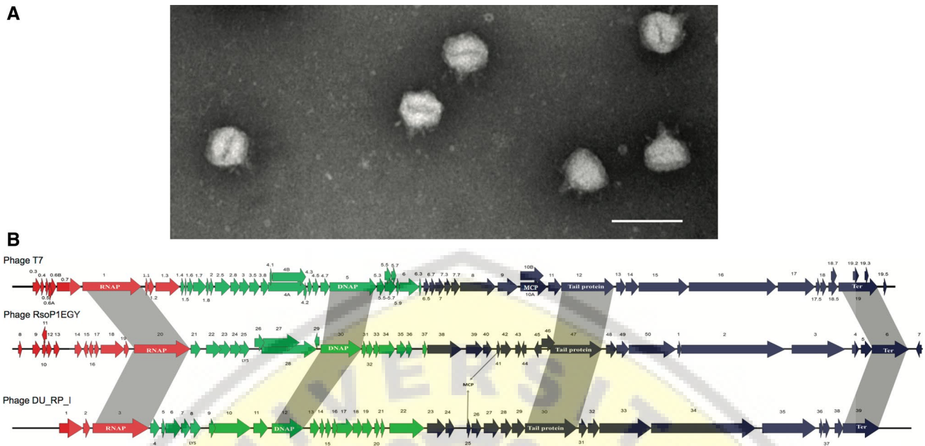
Fig. 1 Electron micrograph of Ralstonia phage RsoP1EGY virions (A) and genome organization of phages RsoP1EGY and DU_RP_I, with reference to the Enterobacteria phage T7 (B). The scale represents 100 nm. Arrows represent the size and direction of transcription of ORFs. Functional gene clusters I for early genes, II for DNA metabolism, and III for virion structure and assembly of phages
