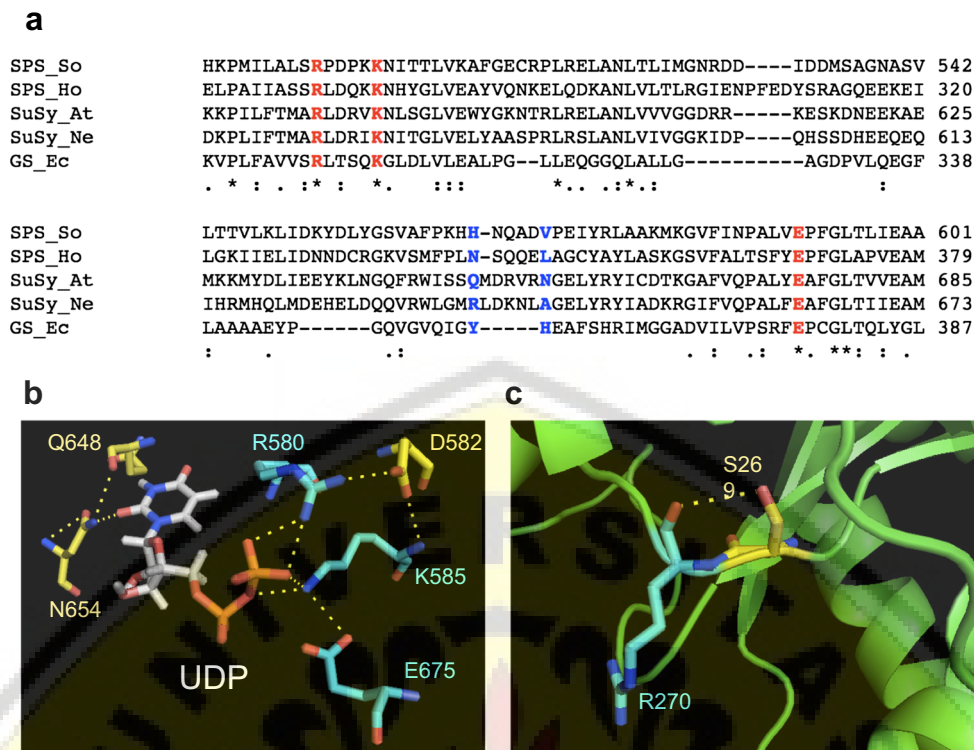
Fig. 1 Comparison of residues in glycosyltransferases group. a Multiple sequence alignment of SPS in sugarcane ( So SPS1), SPS in non-photosynthetic bacterial H. orenii ( Ho SPS), sucrose synthase in A. thaliana ( At SuSy), sucrose synthase in bacteria N. europaea ( Ne SuSy), and glycogen synthase from E. coli ( Ec GS). The three highly conserved and critical residues that consist of arginine, lysine, and glutamic acid are shown in red. The residues that are predicted to be involved in nucleotide
