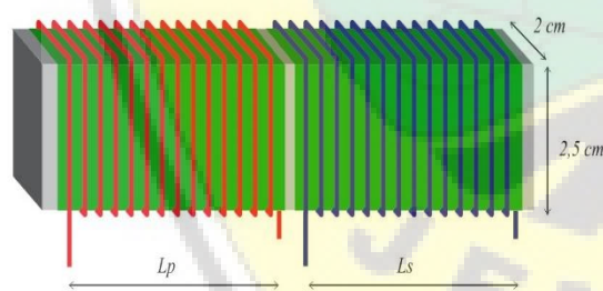
FIGURE 3. Coil Design
