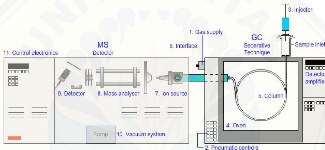
Gambar 2.5. GC-MS ( Gas Chromatography Mass Spectrometry ) (Anonim, 2017).
