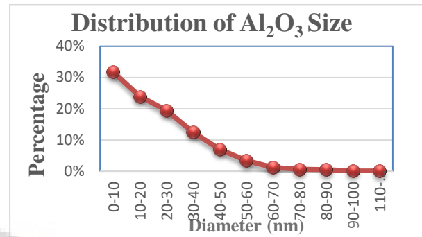
Figure-9. Distribution of alumina nanoparticle size on HSS electrodes.
