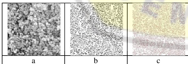
Figure-8. Processing the resulting images of the alumina particle SEM of HSS electrodes using Image J (a) alumina nanoparticle; (b) Thresholding; (c) Outlines.
