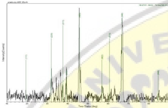
Figure-11. Results using XRD on HSS electrode nanoparticle.
