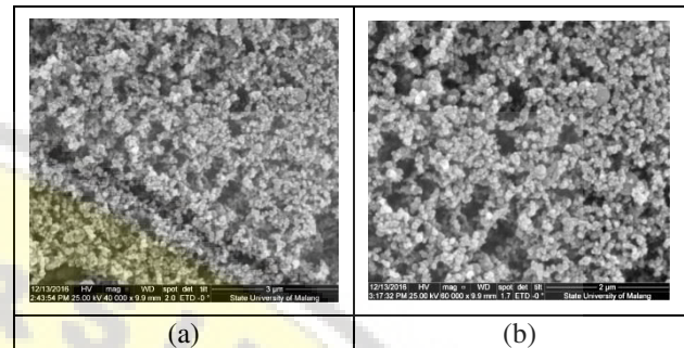
Figure-4. SEM results of alumina particles with copper electrodes (a) magnification 40.000x; (b) magnification 60.000x
