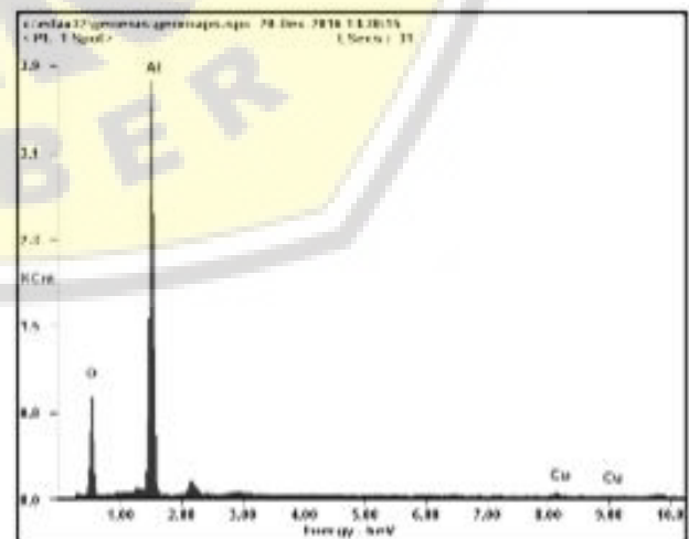
Figure-10. Results of energy dispersive X-ray (EDX) on alumina nanoparticles.
