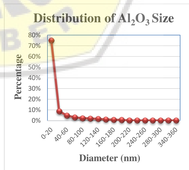
Figure-6. Distribution of alumina nanoparticle size on copper electrodes.
