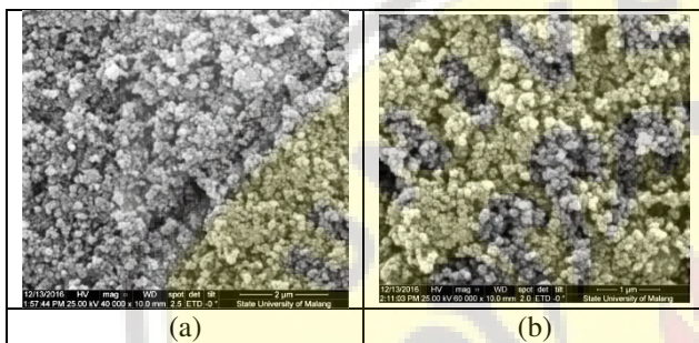
Figure-7. SEM results of alumina particles with HSS electrodes (a) magnification 40.000x; (b) magnification 60.000x.
