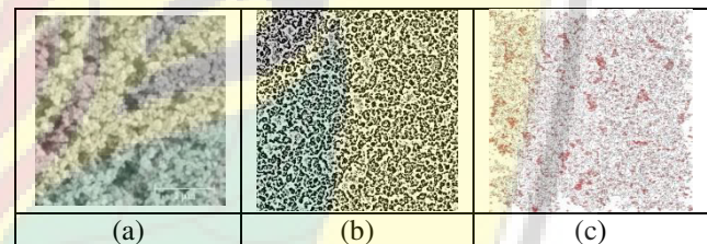
Figure-5. Processing the resulting images of the alumina particle SEM of copper electrodes using Image J (a) alumina nanoparticle; (b) Thresholding; (c) Outlines.
