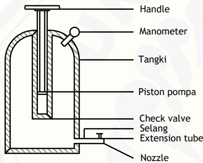
Gambar 6.1 Automatic Sprayer
