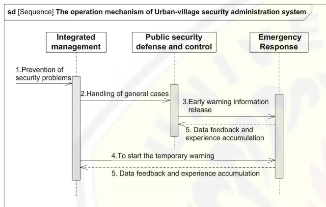
Fig.1. SysML Sequence Diagram of Operation Mechanism
