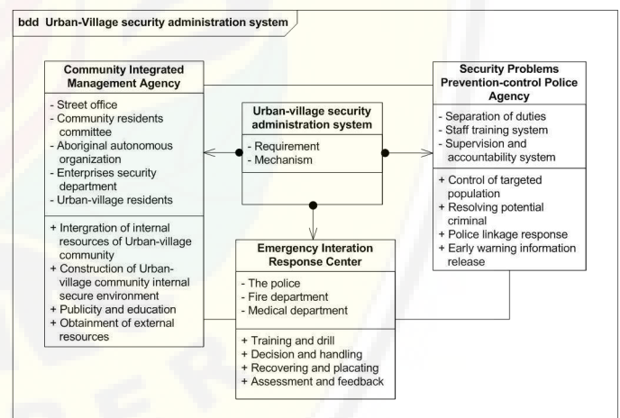
Fig.3. SysML Class Diagrams of Security Management System
