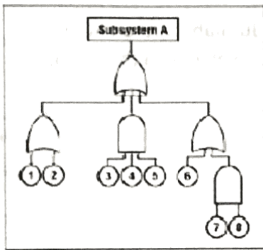
Gambar 1. Gambaran Diagram Fault Tree
