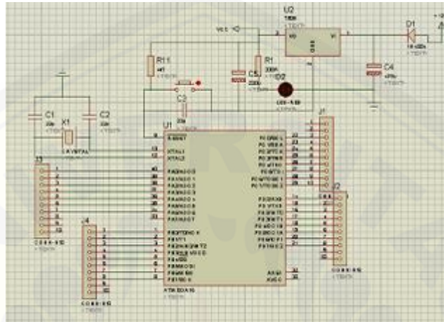
Gambar 2.1 Minimum sistem
