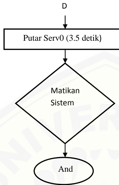
Gambar 3.14 Flowchart
