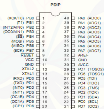
Gambar 2.2 Chip Mikrokontroler Atmega16
