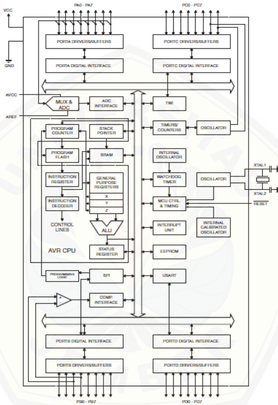
Gambar 1.3 diagram block ATmega 32
