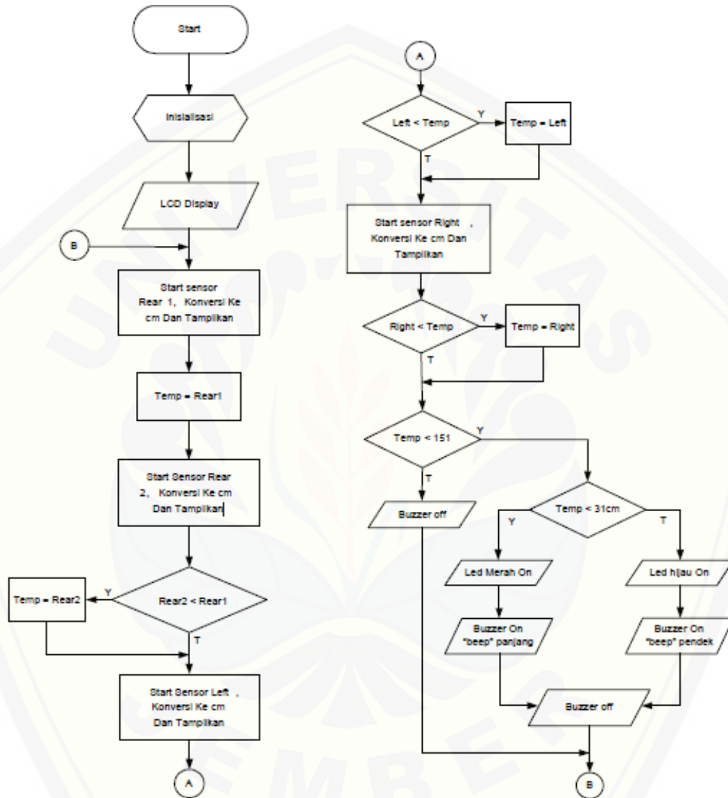
Gambar 2.4 Flowchart
