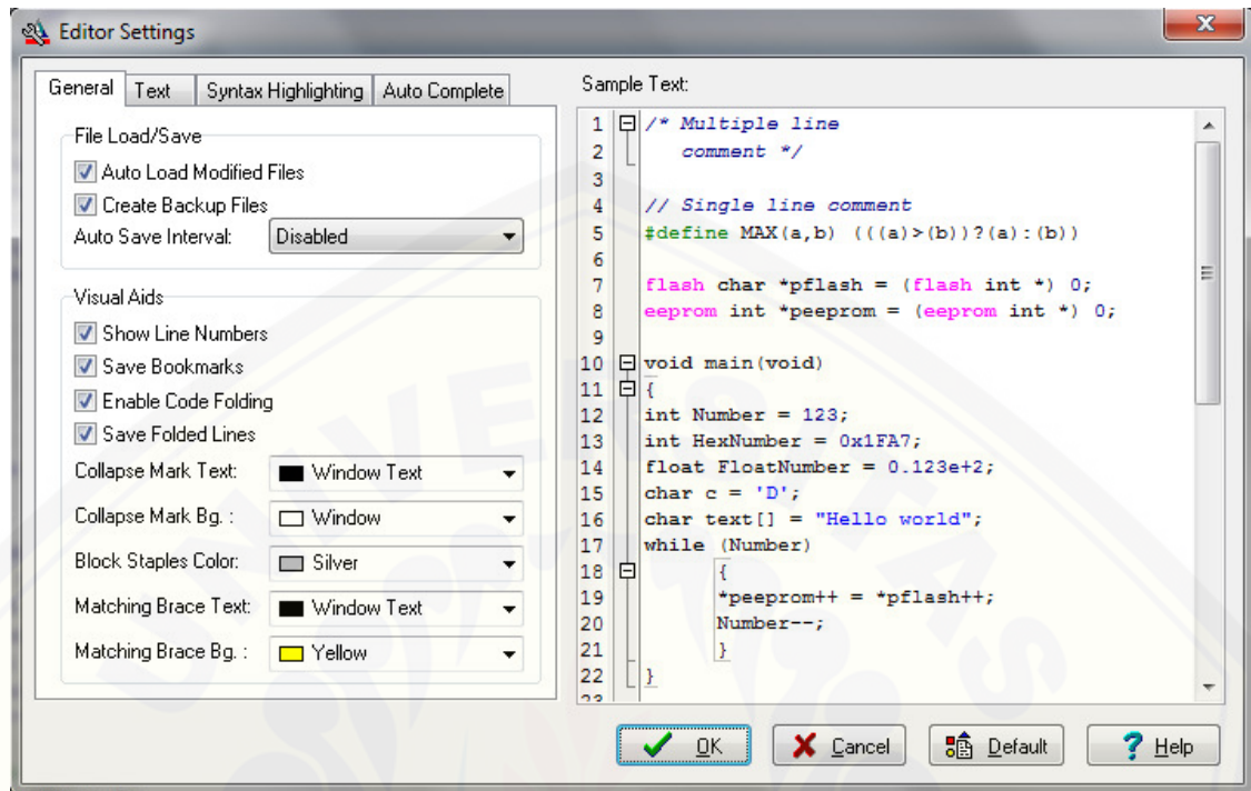
Gambar 2.1 editor codevision-AVR
