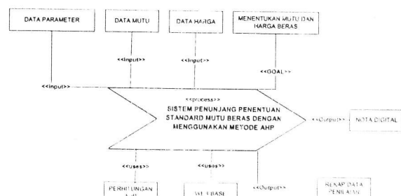
Gambar 1. Business Process
