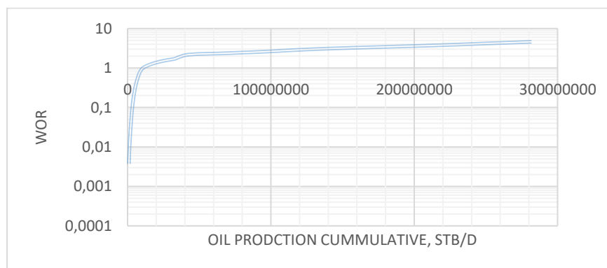
Gambar 4.25 Hasil WOR Plot
