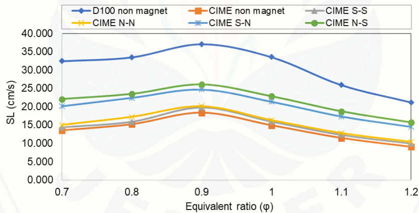
Figure 5. Laminar flame speed of premixed fuel D100 and CIME biodiesel with the effect of magnetic field
