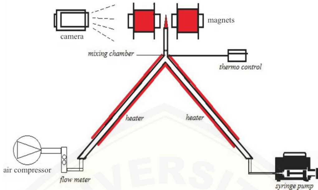
Figure 2. Experiment setup
