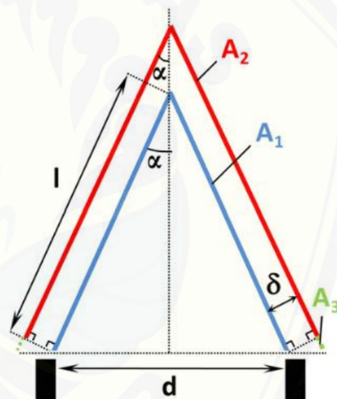
Figure 3. Illustration of cone bunsen flame angle [36], [37]
