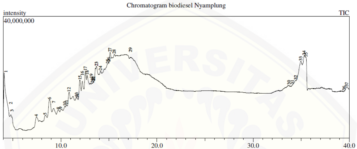
Figure 1. GCMS of CIME biodiesel
