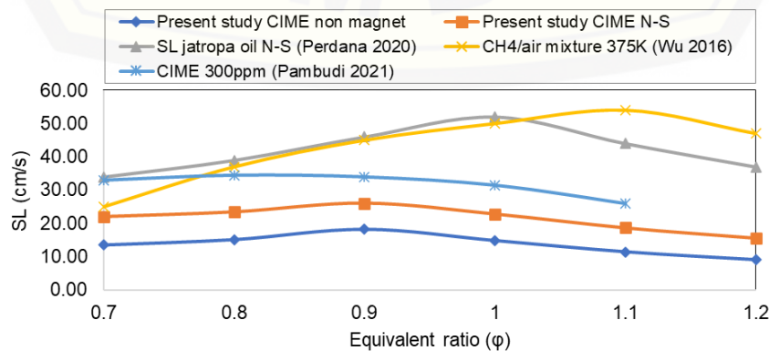
Figure 6. Laminar flame speed: current and previous experiments
