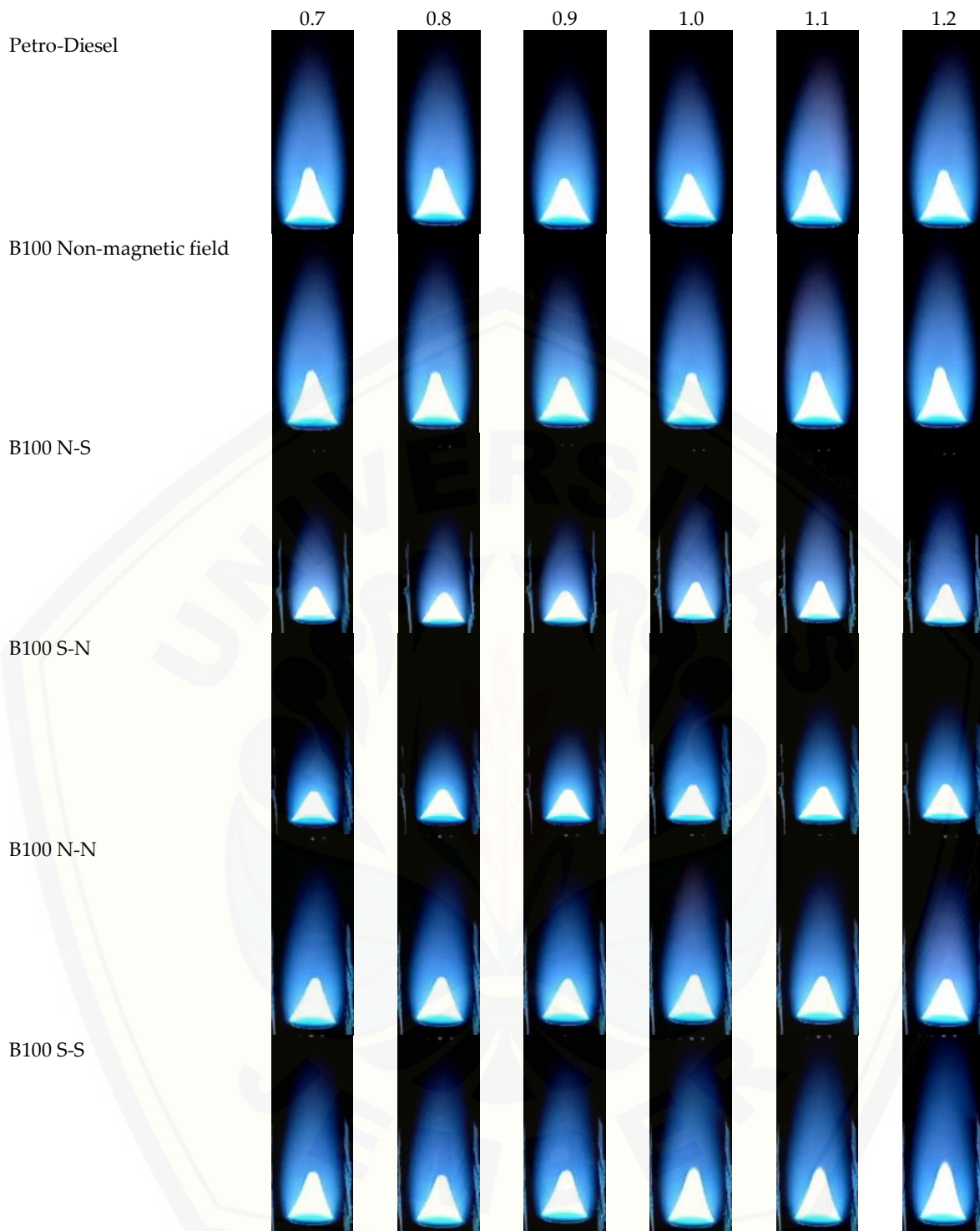
Figure 4. Flame with magnetic fields variation and equivalent ratio
