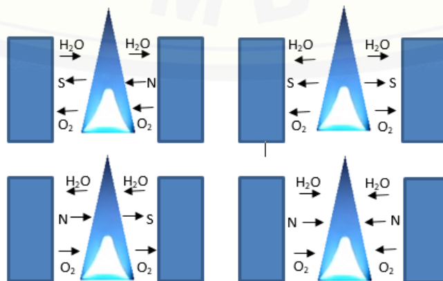
Figure 7. Movement illustration of O_2 and H_2O due to influence of a magnetic field
