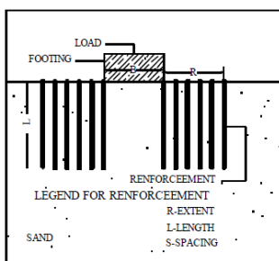
Fig. 4. Bamboo pile plan for footing reinforcement (adapted from [36]).
