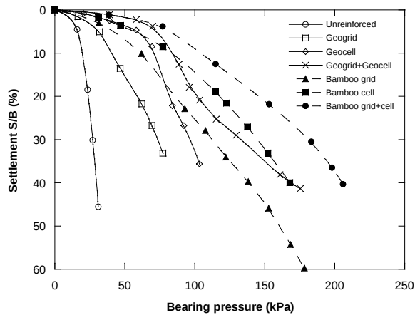
Fig. 2. Bearing pressure – settlement curves for various reinforcement (adapted from [19])
